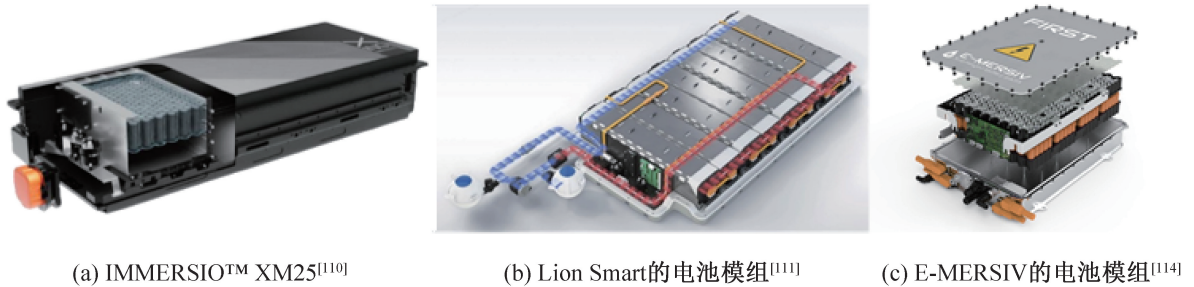
图 10 浸没液冷电池模组 Fig.10 Immersion liquid-cooled battery module
