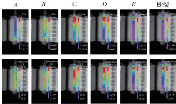
图4 DIC获得的轴向应变与IR获得的表面温度的演化过程 Fig.4 Evolution of axial strain obtained by DIC and surface temperature obtained by IR
