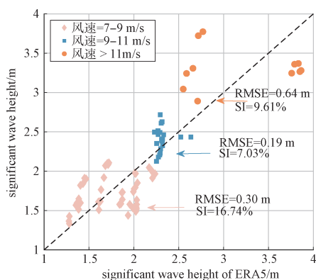
图5 SWOT数据反演的有效波高与ERA5有效波高对比图 Fig. 5 The comparison of the significant wave height retrieved from SWOT data with the ERA5 significant wave height
