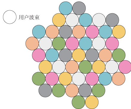
图7 跳波束用户波束均匀分簇布局示意图B Fig. 7 Illustration B of the uniform clustering layout of the beam hopping user of the beam hopping user
