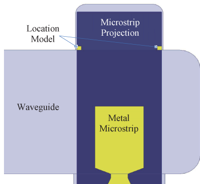
(a) 悬置微带的新型结构模型 (a) New structure of suspended microstrip
