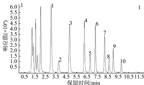
注: 1. PFOA; 2. PFHxS(全氟己烷磺酸, perfluorohexanesulfonate); 3. PFNA(全氟壬酸, perfluorononanoic acid); 4. PFDA(全氟癸酸, perfluorodecanoic acid); 5. PFOS; 6. PFUDA(全氟十一酸, perfluoroundecanoic acid); 7. PFDDA(全氟十二酸, perfluorododecanoic acid); 8. PFDS(全氟癸烷磺酸, perfluorodecanesulfonate); 9. PFTrDA(全氟十三酸, perfluorotridecanoic acid); 10. PFTEDA(全氟十四酸, perfluorotetradecanoic acid)。
