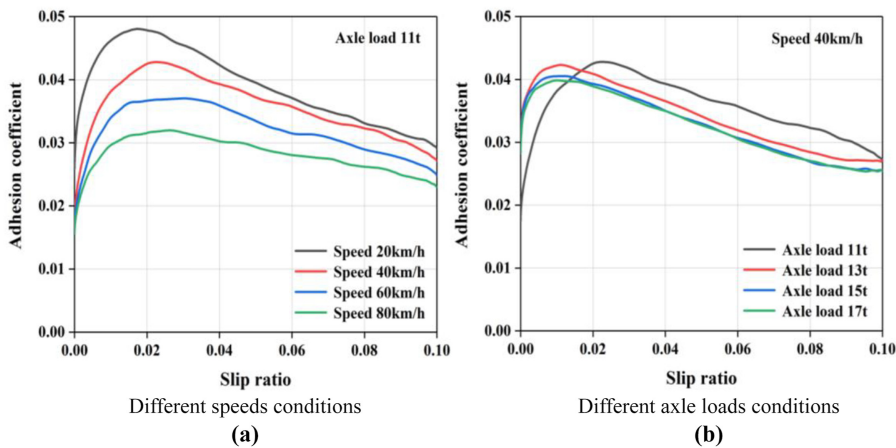
Figure 4. The adhesion coefficient-slip ratio curves under oil-water mixed medium small creepage conditions
