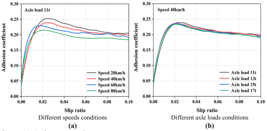
Figure 2. The adhesion coefficient-slip ratio curves under water medium small creepage conditions
