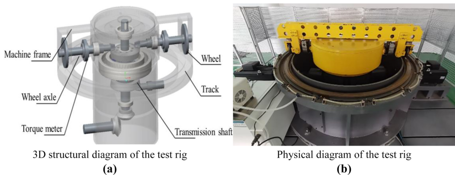
Figure 1. The PLS-160 wheel-rail adhesion simulation test rig
