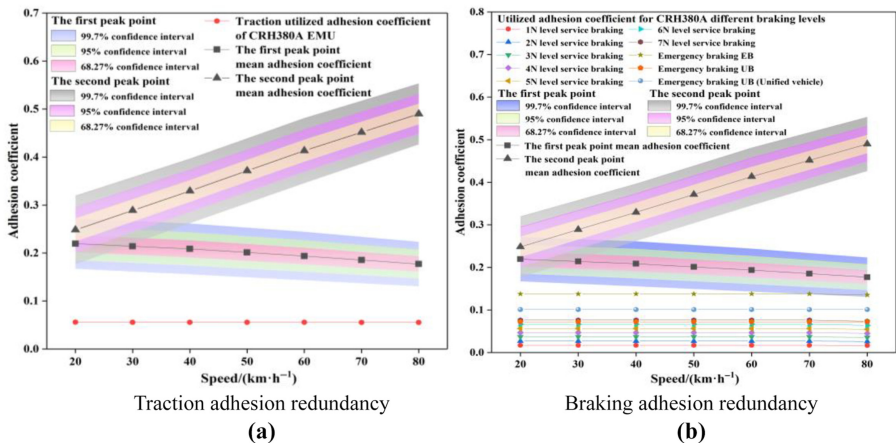
Figure 15. Analysis diagram of wheel-rail adhesion redundancy under water medium large slip conditions
