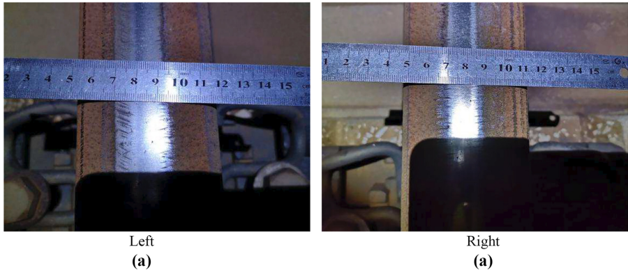
Figure 6. Wheel–rail contact band of the 60N rail
