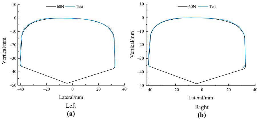
Figure 5. Tested profiles of 60N rail compared with 60N profile
