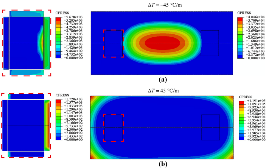
Note(s): (a) Contact stress of the slab when \Delta T = -45 \text{ }^\circ\text{C/m} ; (b) contact stress of the slab when \Delta T = 45 \text{ }^\circ\text{C/m}
