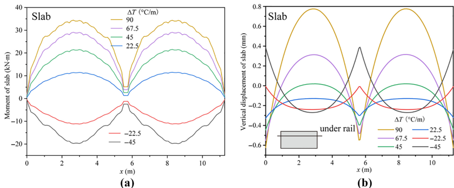
Figure 3. Initial periodic deformation and its mechanical origin of the slab under different temperature gradients
