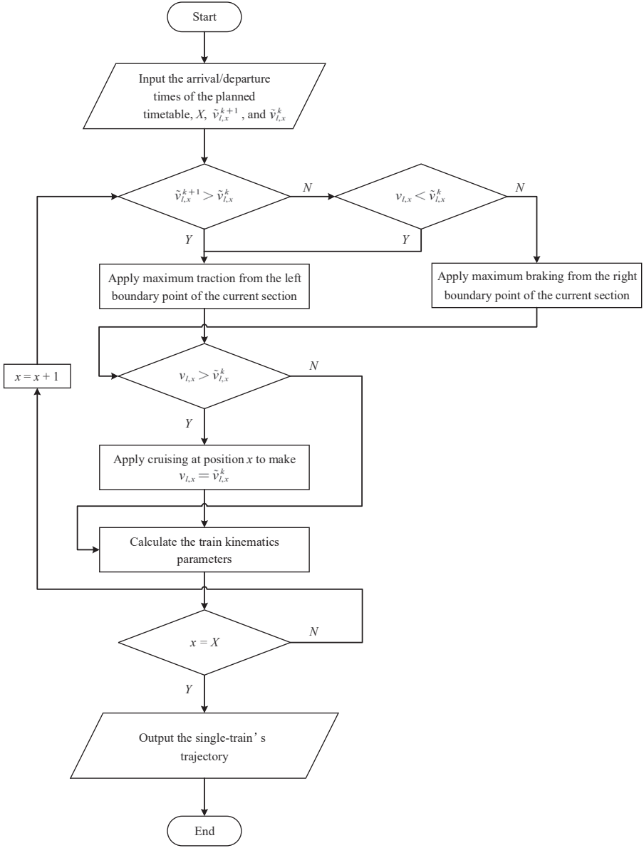
Figure 2. Flow chart of the STTO algorithm
