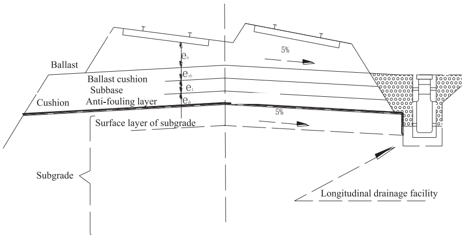
Figure 9. Structure of subgrade bed for high speed railways in France
