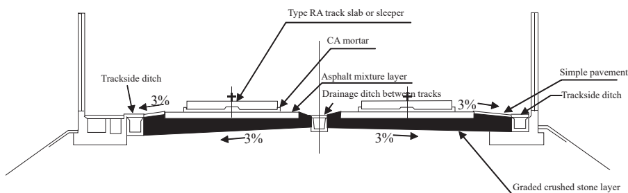
Figure 2. Schematic cross section of asphalt surface layer of subgrade bed for ballastless tracks in Japan
