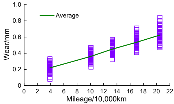
Tread wear changing with service mileage
