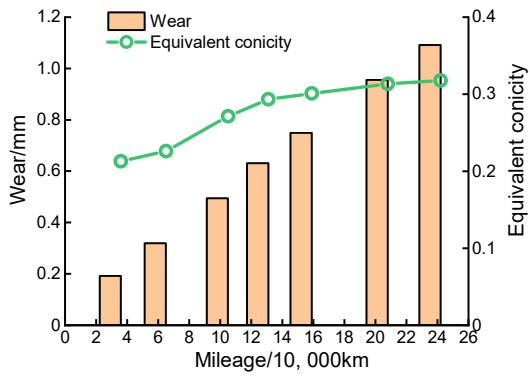
Harbin-Dalian HSR (c)
