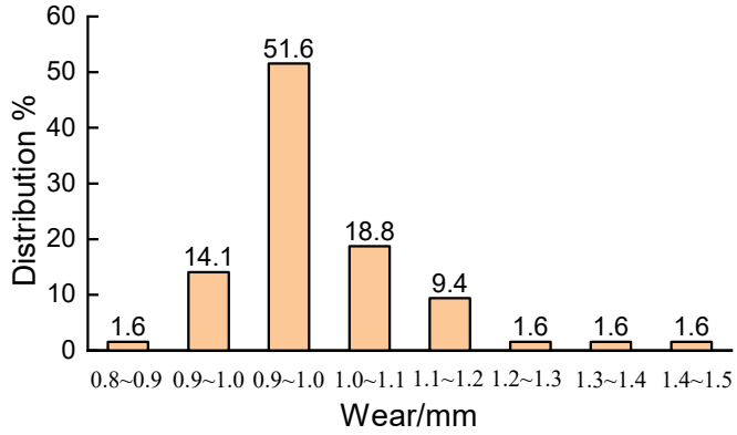
Statistics of tread wear at the end of a reprofiling cycle
