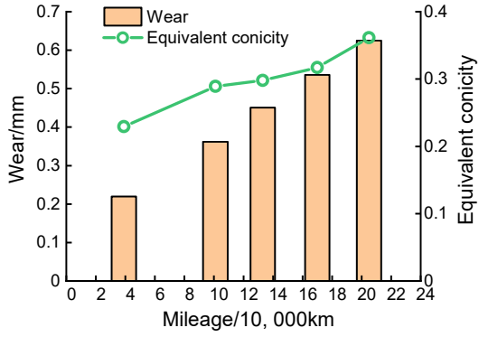
Beijing-Shanghai HSR (a)
