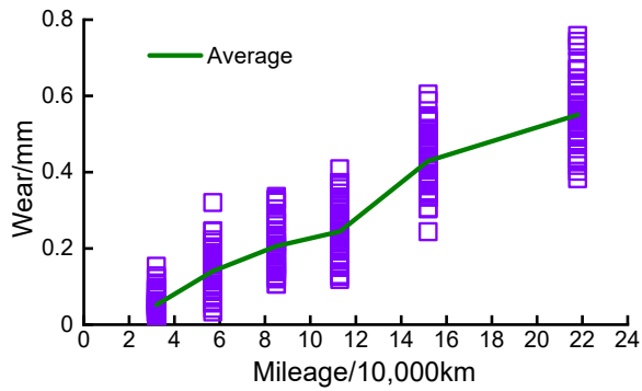
Tread wear changing with service mileage (a)
