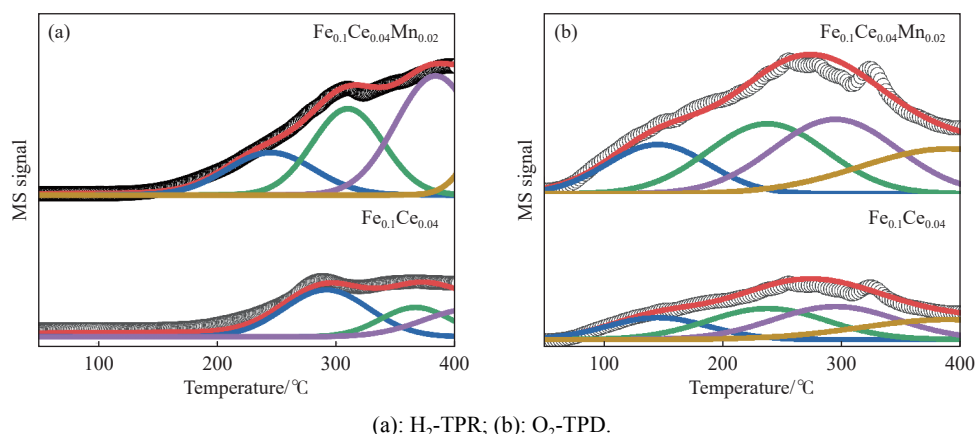
图 6 \text{Fe}_{0.1}\text{Ce}_{0.04} 与 \text{Fe}_{0.1}\text{Ce}_{0.04}\text{Mn}_{0.02} 催化剂的 \text{H}_2 -TPR 与 \text{O}_2 -TPD 表征 Fig. 6 \text{H}_2 -TPR and \text{O}_2 -TPD profiles of \text{Fe}_{0.1}\text{Ce}_{0.04} and \text{Fe}_{0.1}\text{Ce}_{0.04}\text{Mn}_{0.02} catalysts
