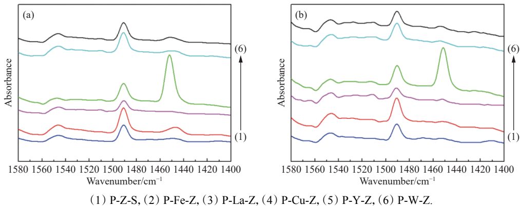
图 2 水热处理后改性 ZSM-5 分子筛的吡啶吸附红外光谱谱图 Fig. 2 Pyridine adsorption FT-IR spectra of modified ZSM-5 molecular sieves by hydrothermal treatment (Pyridine adsorption FT-IR spectra at (a) 200 and (b) 350 °C)
