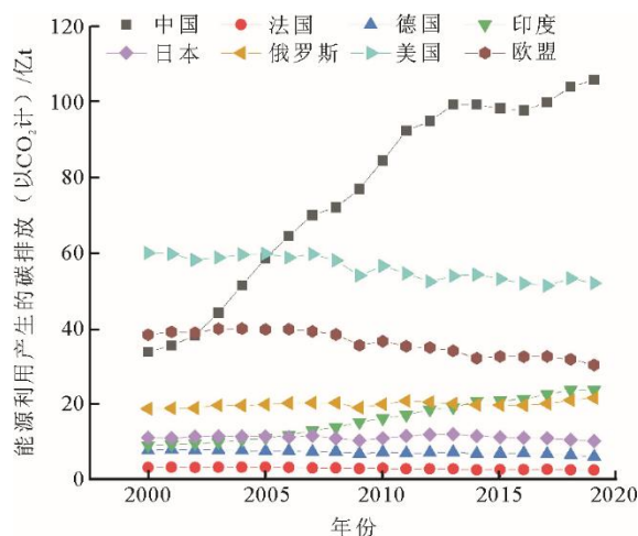
图2 世界各国能源利用产生碳排放量变化 Fig.2 Changes in carbon emissions from energy production in countries around the world
