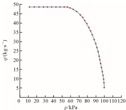
图4 流量-压力变化曲线 Fig.4 Mass flow-pressure curve
