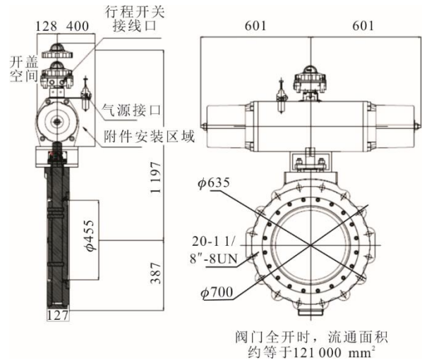
图 1 真空破坏阀结构 (mm) Fig.1 Structure of vacuum breaker valve(mm)
