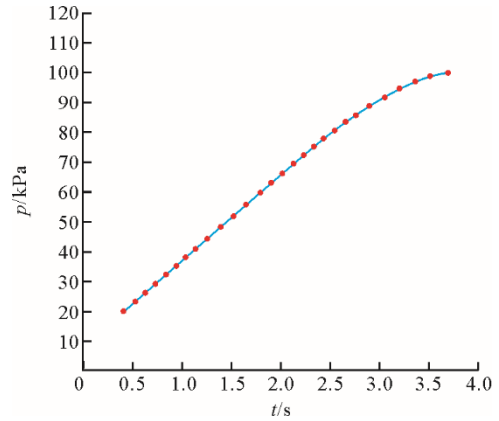
图5 凝汽器内压力-进汽时间曲线 Fig.5 Pressure-admission time curve in condenser
