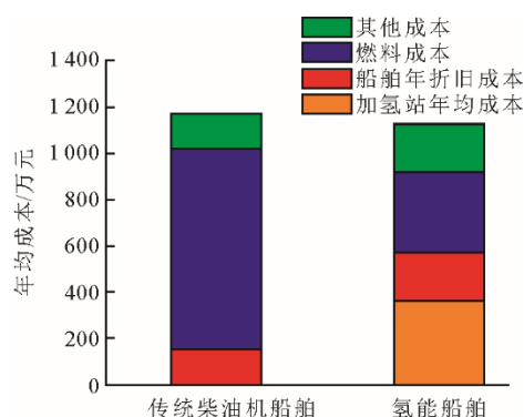
图 2 传统柴油机船舶与氢能船舶年均成本对比 Fig.2 Average annual cost of a conventional diesel ship versus a hydrogen ship
