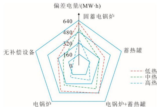
图 6 在不同热量下机组配置不同供热补偿设备调峰空间 Fig.6 The output power range for the plant with different heat compensation equipment
