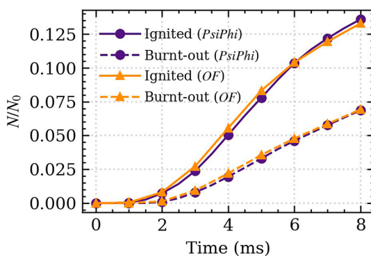
Fig. 4. Temporal evolution of the number of particles that are ignited and burnt-out from the present simulation and from the work by Luu et al. (2024a).
