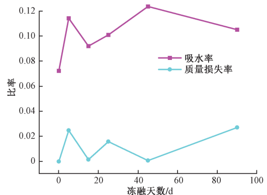
图10 酸性环境质量损失率与吸水率 Fig.10 Acid environmental quality loss rate and water absorption rate
