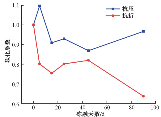
图9 酸性环境软化系数 Fig.9 Softening coefficient in acid environment
