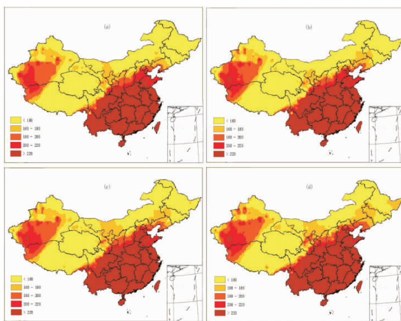
(a) 1964–1973 年我国无霜期均值分布图; (b) 1974–1983 年我国无霜期均值分布图; (c) 1984–1993 年我国无霜期均值分布图; (d) 1994–2003 年我国无霜期均值分布图 (a) Distribution of FFD from 1964 to 1973; (b) Distribution of FFD from 1974 to 1983; (c) Distribution of FFD from 1984 to 1993; (d) Distribution of FFD from 1994 to 2003
