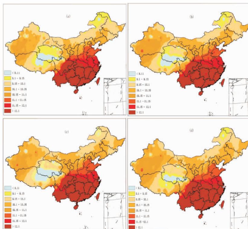
(a) 1964–1973 年我国初霜日均值分布图; (b) 1974–1983 年我国初霜日均值分布图; (c) 1984–1993 年我国初霜日均值分布图; (d) 1994–2003 年我国初霜日均值分布图 (a) Distribution of FFD from 1964 to 1973; (b) Distribution of FFD from 1974 to 1983; (c) Distribution of FFD from 1984 to 1993; (d) Distribution of FFD from 1994 to 2003
