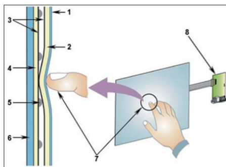
(a) 电阻式触摸屏
