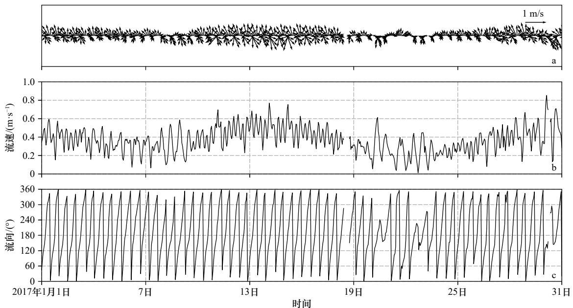
图6 2017年1月流速矢量时间序列(a)、流速时间序列(b)和流向时间序列(c) Fig. 6 Time series of tidal current vector (a), time series of tidal current velocity (b), and time series of tidal current direction (c) in January, 2017
