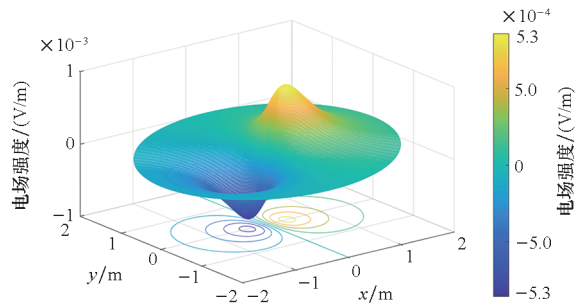
(a) E_x
