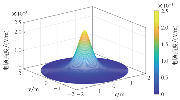
(c) E_z
