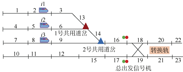
图 1 车辆场段布线示意 Figure 1 Schematic of the depot
