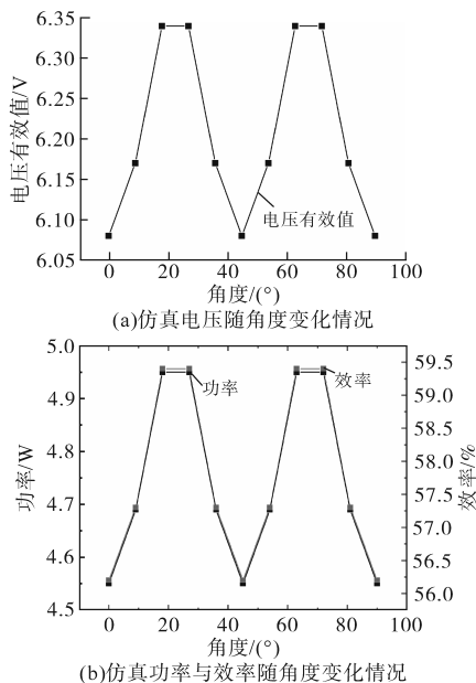
图11 两接收线圈的电压、功率与效率随角度变化情况 Fig.11 The voltage, power and efficiency of two receiver coils as a function of angle
