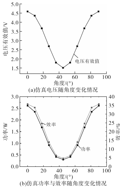
图10 单接收线圈的电压、功率与效率随角度变化情况 Fig.10 The voltage, power and efficiency of a single receiver coil as a function of angle
