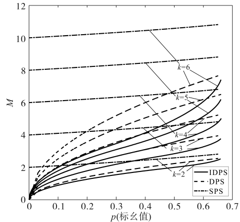
图5 三种调制方式下的最小电流应力对比曲线 Fig.5 Comparison curve of minimum current stress under three modulation modes
