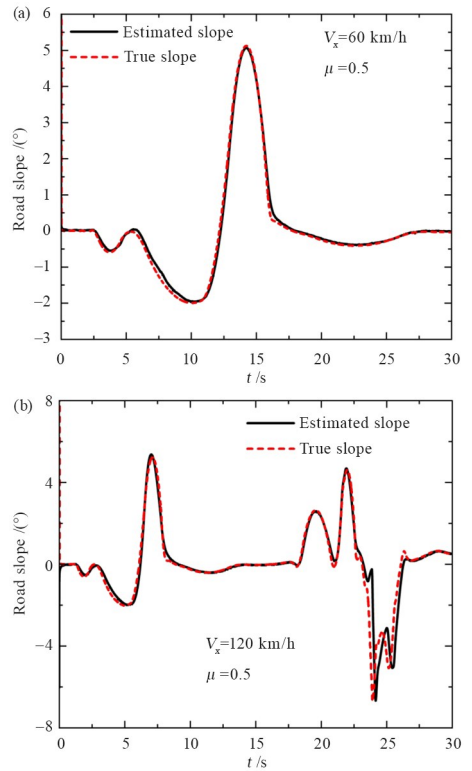
图 10 双移线工况( \mu = 0.5 )的变坡度估算结果: (a)RMSE = 0.6736^\circ ; (b)RMSE = 1.4121^\circ
