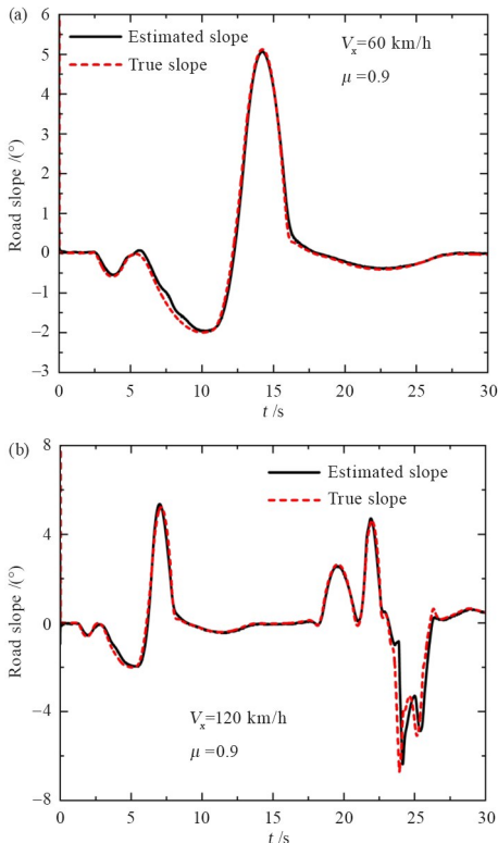
图 9 双移线工况( \mu = 0.9 )的变坡度估算结果: (a)RMSE = 0.6724^\circ ; (b)RMSE = 1.3334^\circ
