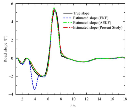
图 4 已有研究与本文方法的坡度估算结果对比 Fig. 4 Comparison of road slope estimation results between previous studies and the present study
