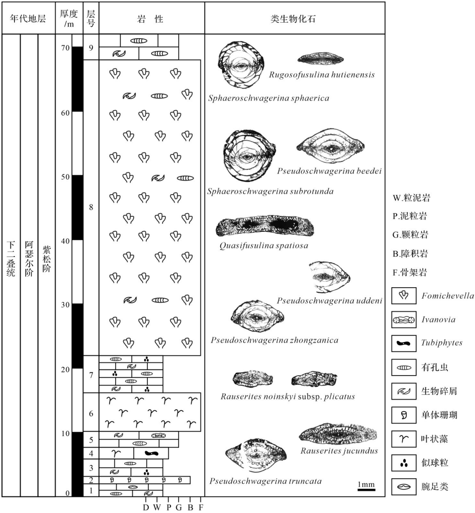
图3 窝托村珊瑚礁剖面柱状图 Fig.3 Stratigraphic column of the coral reef section, Wotuo village
