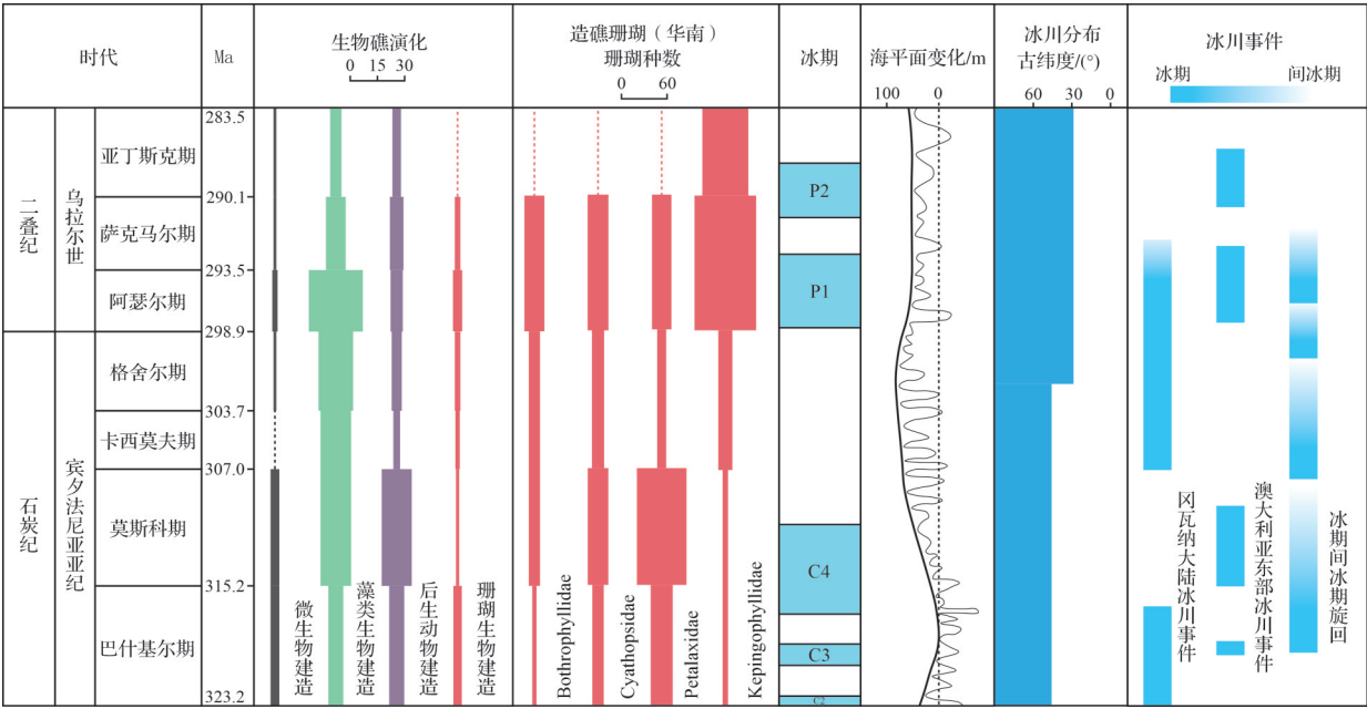
图 10 宾夕法尼亚亚纪—乌拉尔世生物礁演化与晚古生代冰期对比(据 Crowley and Baum, 1992; Wang et al. , 2006; Rygel et al. , 2008; Chen et al. , 2016; Kiessling and Krause, 2022)
