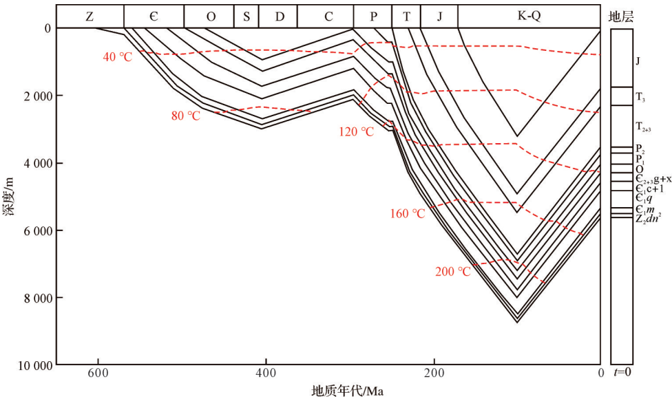
图10 川中GS17井埋藏史图(据杨程宇等,2020修改) Fig.10 Burial history of well GS17, central Sichuan Basin (modified from Yang et al. , 2020)
