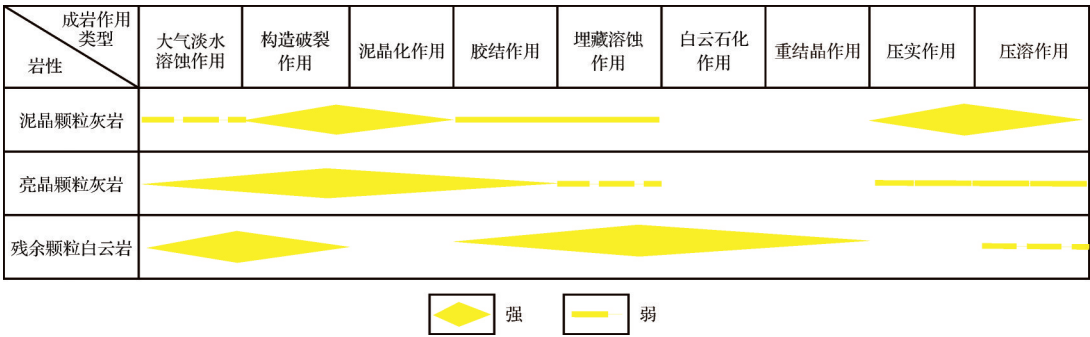
图9 研究区栖霞组各岩类成岩作用发育情况 Fig.9 Diagenetic development of each rock type from the Qixia Formation in the study area
