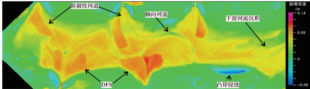
图10 新增砂体平面展布 Fig.10 Planar spreading of added sand bodies
