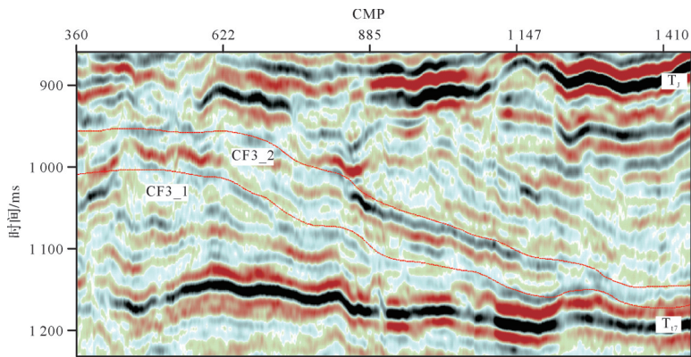
图 11 地震剖面(红线为解释层位) Fig.11 Seismic profile (red line represents the horizon interpretation)
