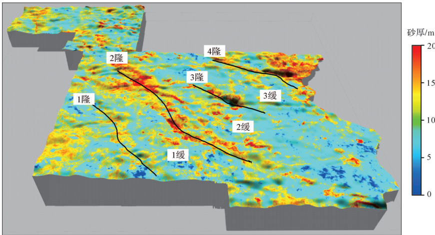
图 13 陇东地区沉积期湖盆构造与长 7 3 亚段砂厚叠合图 Fig.13 Stacking map of the bottom shape of the lake basin during the sedimentary period and Chang 7 3 sub-member sand thickness in the Longdong area
