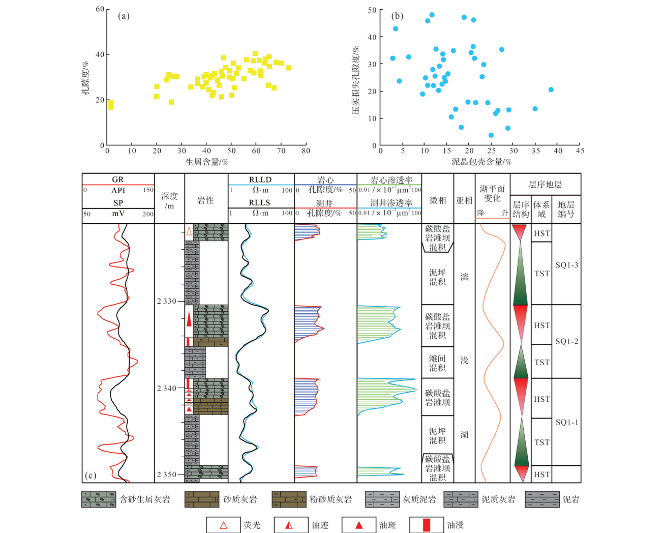
图9 混合沉积与优质储层关系 (a)生屑含量与孔隙关系;(b)泥晶包壳含量与压实损失孔隙度的关系;(c)G118井,储层特征(2 330.6~2 343.4 m) Fig.9 Relationship between mixed sedimentation and high-quality reservoirs
