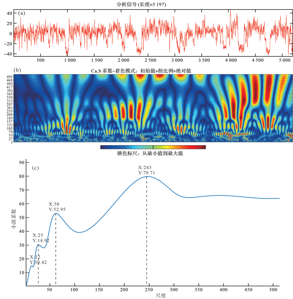
图6 仙中39井测井信号小波变换 (a)预处理之后仙中39井测井GR数据;(b)小波变换能量图谱;(c)小波变换模均值曲线 Fig.6 Wavelet transform of well logging signals in well Xianzhong 39 (a) gamma ray (GR) data after preprocessing; (b) wavelet transform energy spectrum; (c) wavelet transform modulus mean curve
