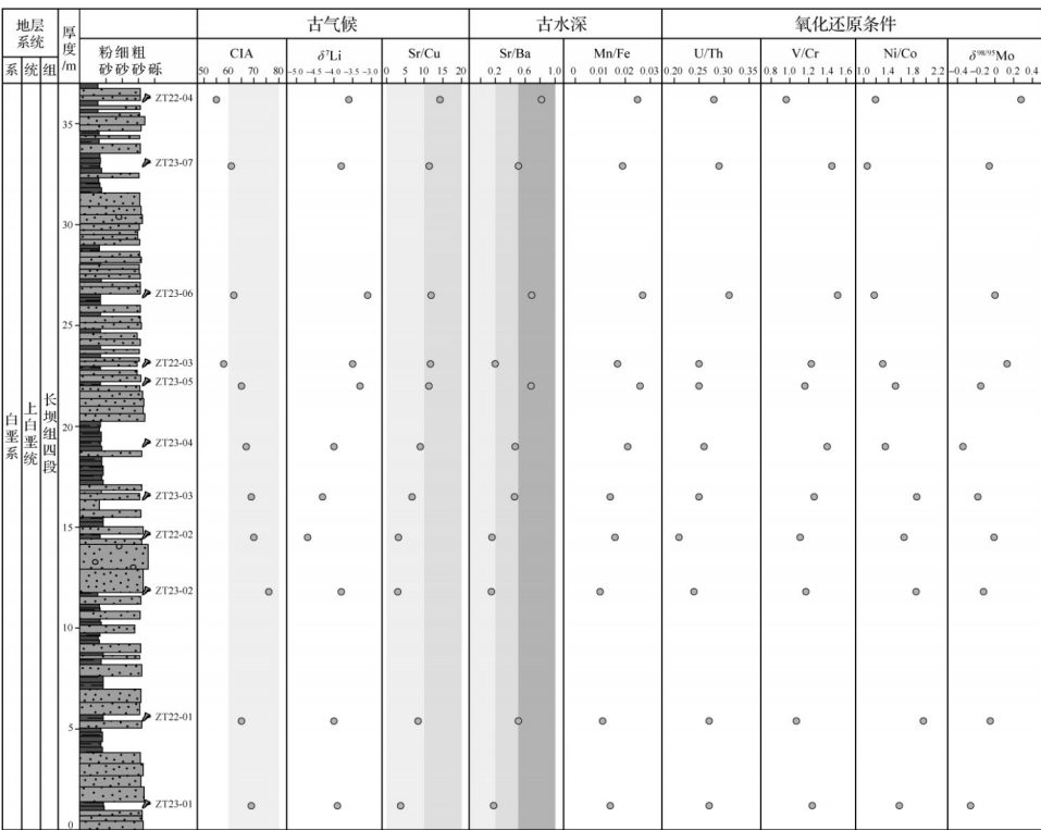
图9 丹霞盆地上白垩统长坝组四段细粒碎屑岩地球化学指标垂向变化特征 Fig.9 Geochemical indicators of fine-grained clastic rocks in the Fourth member of the Changba Formation, Upper Cretaceous, Danxia Basin
