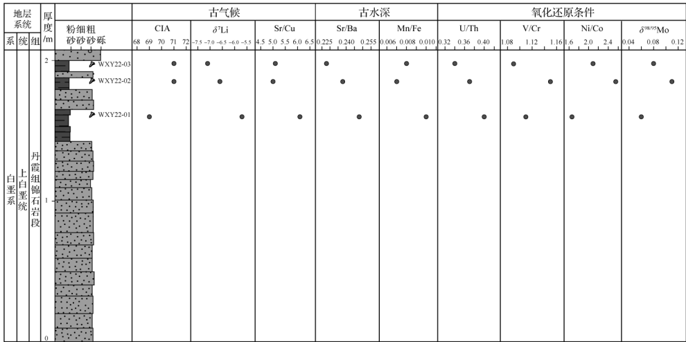
图11 丹霞盆地上白垩统丹霞组锦石岩段(晚秀岩剖面)细粒碎屑岩地球化学指标垂向变化特征 Fig.11 Geochemical indicators of fine-grained clastic rocks in the Jinshiyan member of the Danxia Formation, Upper Cretaceous (Wanxiuyan section), Danxia Basin
