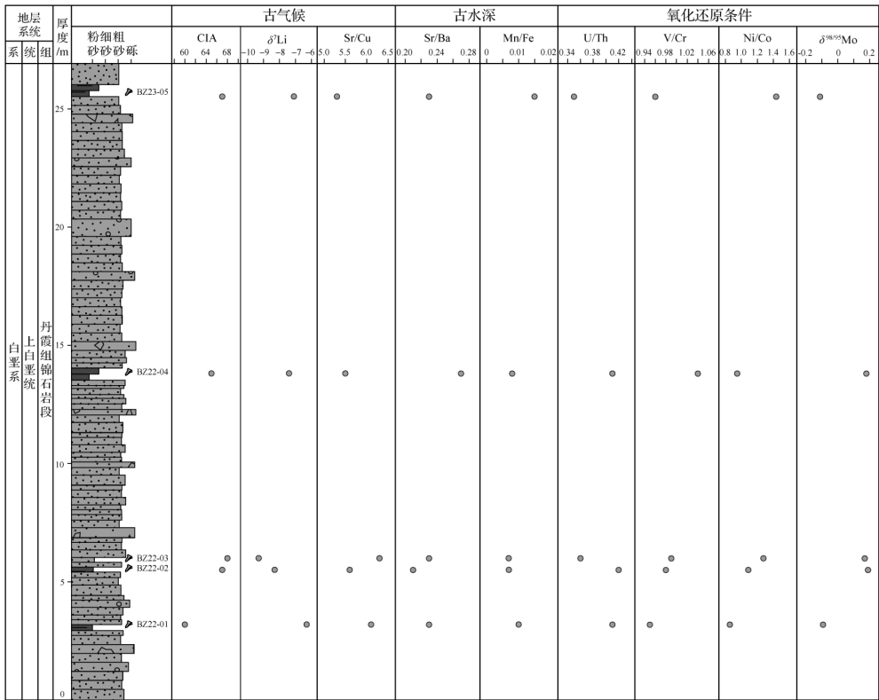
图10 丹霞盆地上白垩统丹霞组锦石岩段(巴塞剖面)细粒碎屑岩地球化学指标垂向变化特征 Fig.10 Geochemical indicators of fine-grained clastic rocks in the Jinshiyan member of the Danxia Formation, Upper Cretaceous (Bazhai section), Danxia Basin
