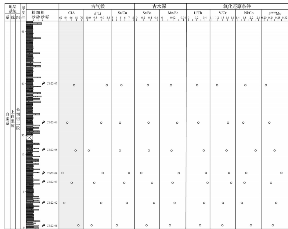
图8 丹霞盆地上白垩统长坝组二段细粒碎屑岩地球化学指标垂向变化特征 Fig.8 Geochemical indicators of fine-grained clastic rocks in the Second member of the Changba Formation, Upper Cretaceous, Danxia Basin
