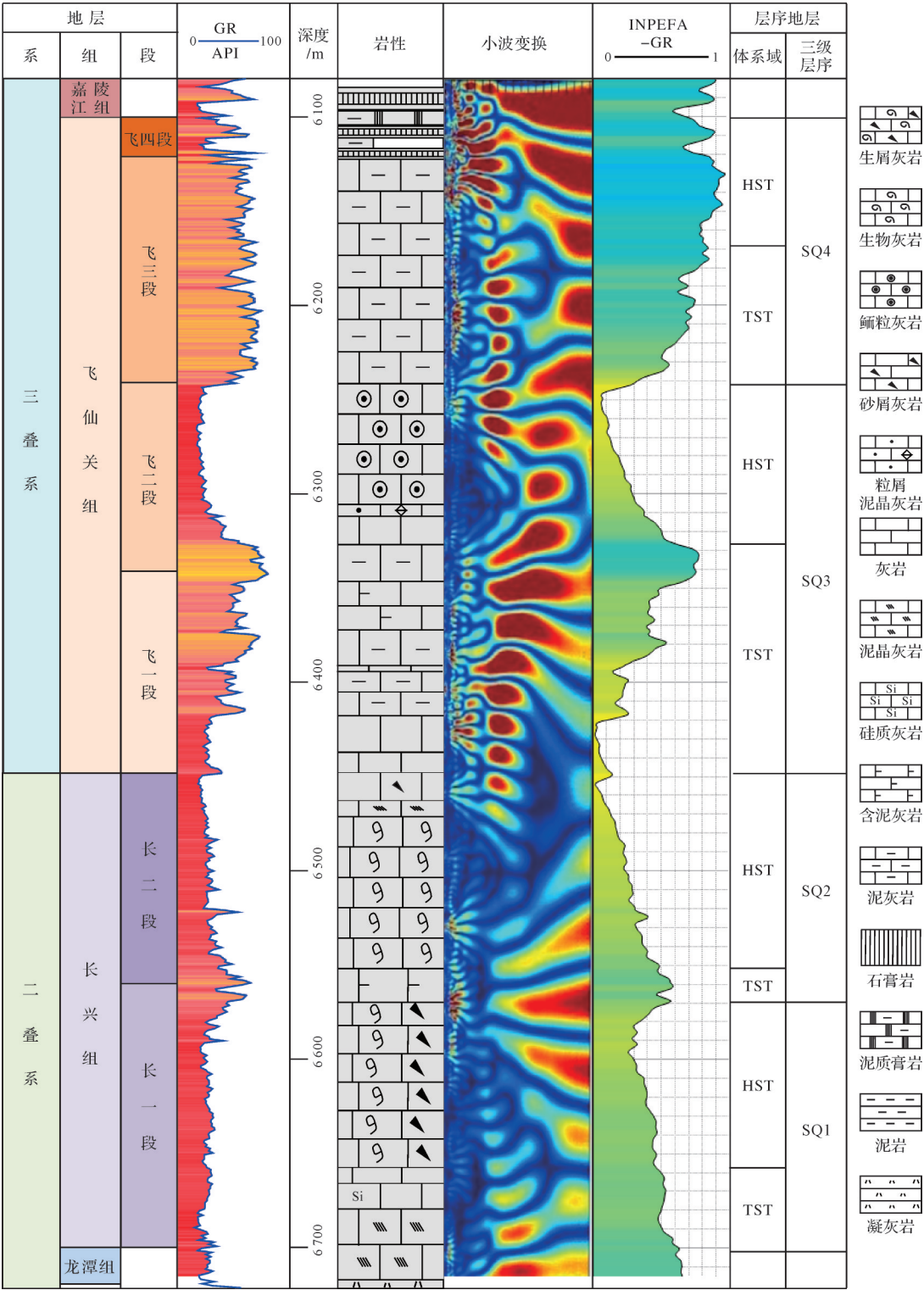
图2 St1井长兴组—飞仙关组层序地层综合柱状图 Fig.2 Sequence stratigraphy comprehensive column of the Changxing Formation-Feixianguan Formation in well St1
