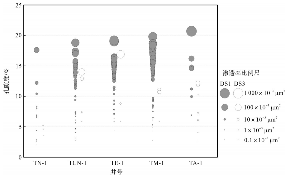
图7 Trakes斜坡上白垩统Donga组DS1和DS3段储层测井孔隙度—渗透率交会图 Fig.7 Cross plot of wireline logging porosity and permeability from the Upper Cretaceous Donga Formation in the Trakes slope
