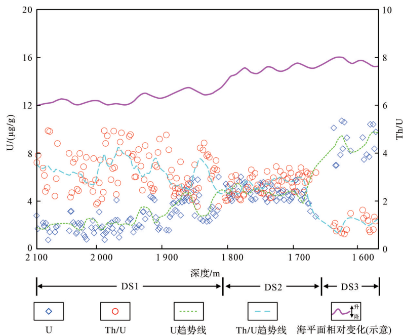
图8 TCN-1井Donga组铀含量(U)和Th/U比值随深度散点分布图 Fig.8 Scatter diagram of uranium content and Th/U with depth for the Donga Formation from well TCN-1
