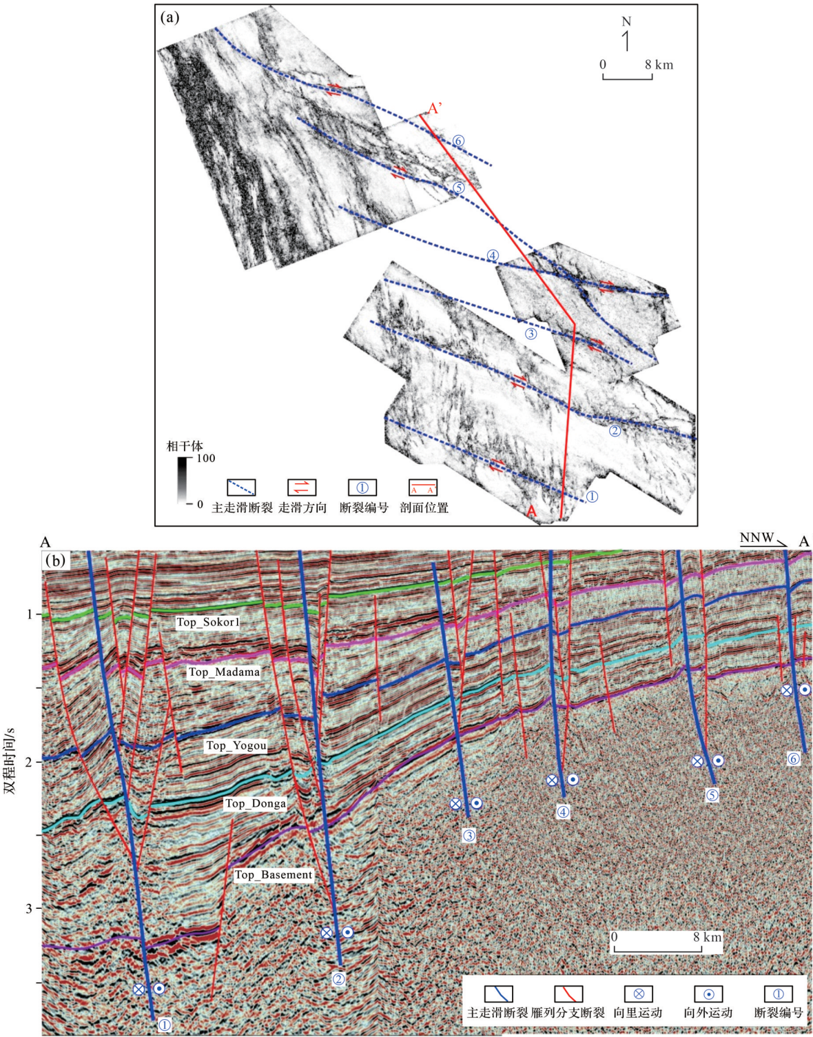
图9 Trakes斜坡Sokor1组顶相干切片图(a)和走滑断裂地震剖面图(b) Fig.9 Coherent body slice (a) and seismic section (b) of strike-slip faults in Trakes slope
