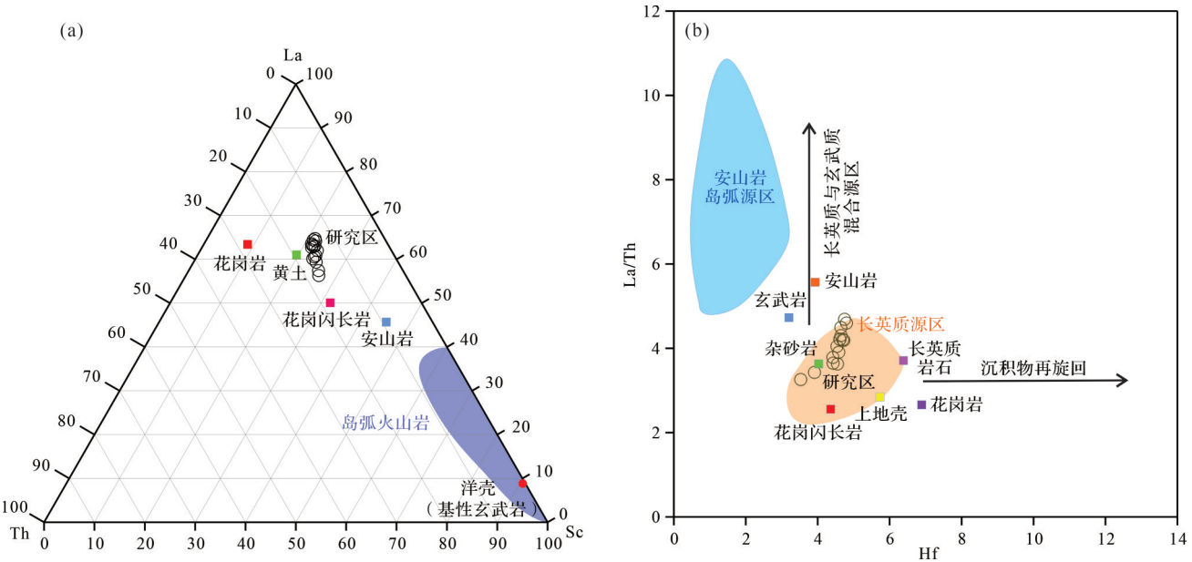
图3 La-Th-Sc 三角图(a)和 La/Th-Hf 双变量图(b)(底图据 Bhatia and Crook, 1986; Floyd and Leveridge, 1987 修改) Fig.3 La-Th-Sc triangle diagram (a) and La/Th-Hf bivariate diagram (b) (base map is modified from Bhatia and Crook, 1986; Floyd and Leveridge, 1987)
