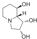
(–)-swainsonine ( 1 )
