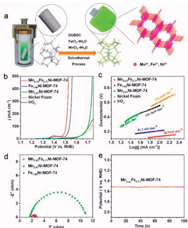
Fig. 15. Synthesis and electrocatalytic performance of \text{Mn}_{0.52}\text{Fe}_{0.71}\text{Ni-MOF-74} on nickel foam (NF). (a) Preparation process of \text{Mn}_{0.52}\text{Fe}_{0.71}\text{Ni-MOF-74} . (b) OER properties. (c) Tafel diagrams. (d) Nyquist diagram. (e) Long-time stability. Reproduced with permission [93]. Copyright 2020, Wiley-VCH.
