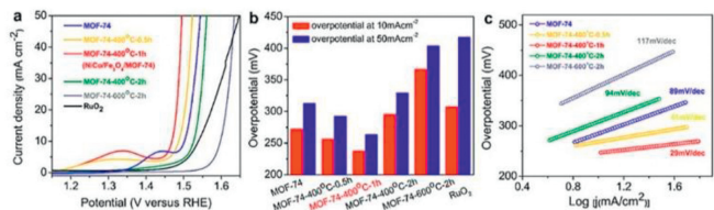
Fig. 16. Electrochemical performances of NiCoFe-MOF-74. (a) LSV curves. (b) The overpotentials at the current density of 10 and 50 mA/cm 2 . (c) Tafel slope. Reproduced with permission [90]. Copyright 2018 ACS.
