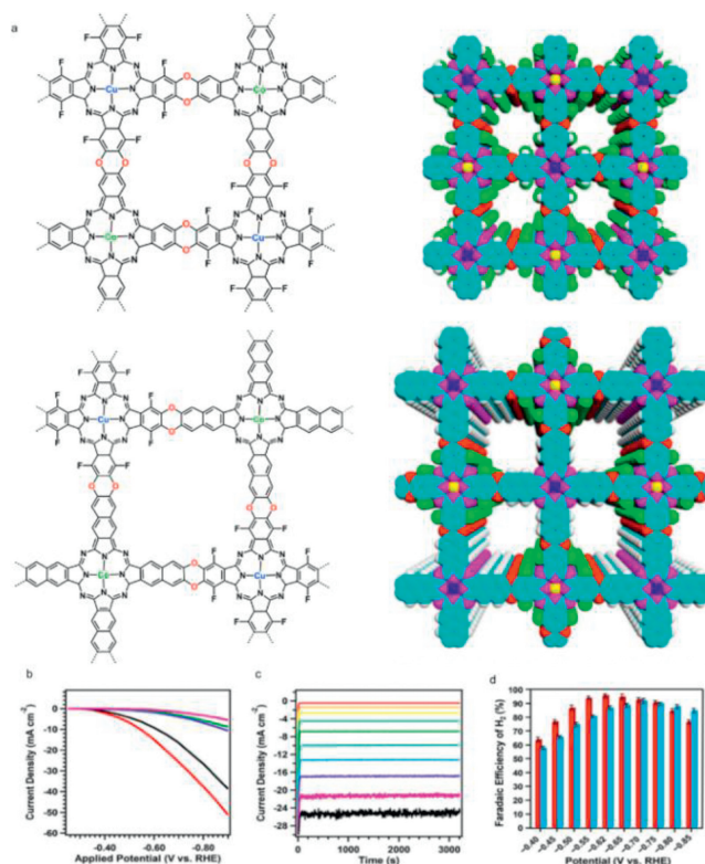
Fig. 23. Schematic illustration and electrocatalytic CO 2 reduction performance of CuPcF 8 -CoPc-COF and CuPcF 8 -CoNPc-COF. (a) Synthesis process. (b) LSV curves of CuPcF 8 -CoPc-COF (black), CuPcF 8 -CoNPc-COF (red). (c) I - t curves of CuPcF 8 -CoNPc-COF at different potentials (from top to bottom: -0.35\text{ V} , -0.38\text{ V} , -0.41\text{ V} , -0.46\text{ V} , -0.50\text{ V} , -0.55\text{ V} , -0.59\text{ V} , -0.63\text{ V} , -0.67\text{ V} , -0.7\text{ V} ). (d) FE CO of CuPcF 8 -CoPc-COF (blue) and CuPcF 8 -CoNPc-COF (red). Reproduced with permission [92]. Copyright 2021, ACS.
