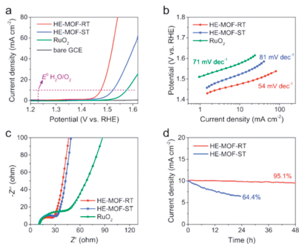
Fig. 18. Electrochemical performance of HE-MOF-RT. (a) LSV polarization curves. (b) Tafel plots. (c) EIS curves. (d) Long-time stability at 10 mA/cm 2 . Reproduced with permission [95]. Copyright 2019, RSC.
