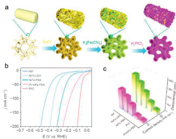
Fig. 17. Synthesis and electrocatalytic performance of Pt-NiFe PBA. (a) preparation process of Pt-NiFe PBA. (b) HER performances in 1 mol/L KOH. (c) Overpotentials at 10 and 50 mA/cm 2 . Reproduced with permission [69]. Copyright 2021, Science Press.
