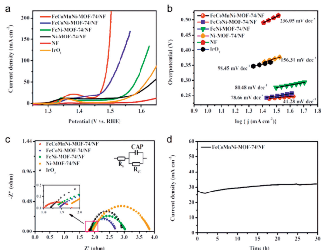
Fig. 22. Electrochemical performance of FeCoMnNi-MOF-74/NF. (a) LSV curves. (b) Tafel diagram. (c) Nyquist plots. (d) Chronoamperometric curve at 1.65 V. Reproduced with permission [72]. Copyright 2021, ACS.
