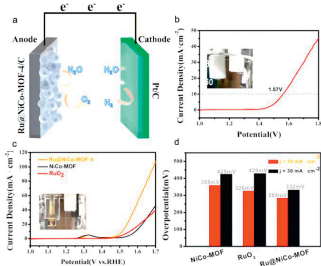
Fig. 25. Electrocatalytic performance of materials. (a) Schematic illustration of water splitting. (b) LSV curve of water splitting. (c) LSV curves. (d) Overpotential required for Ru@NiCo-MOF-4, NiCo-MOF, and commercial \text{RuO}_2 to achieve 10 \text{ mA/cm}^2 and 30 \text{ mA/cm}^2 . Reproduced with permission [119]. Copyright 2021, ACS.
