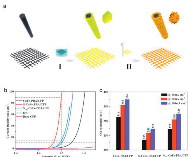
Fig. 11. Synthesis and electrocatalytic performance of materials. (a) Schematic diagram of S-CoFe-PBA/CFP synthesis process. (b) Linear polarization curves. (c) Overpotential at different current density. Reproduced with permission [133]. Copyright 2020, RSC.
