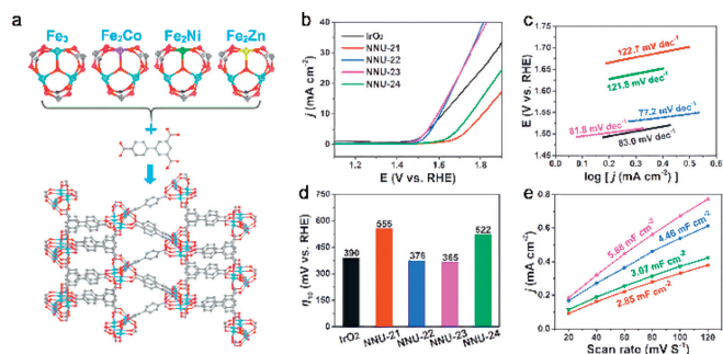
Fig. 14. Crystal structure and electrocatalytic OER performance of NNU-21-24. (a) 3D framework. (b) LSV curves. (c) Tafel plots. (d) Overpotential at 10 \text{ mA/cm}^2 . (e) Plots for C_{dl} . Reproduced with permission [141]. Copyright 2018, Wiley-VCH.
