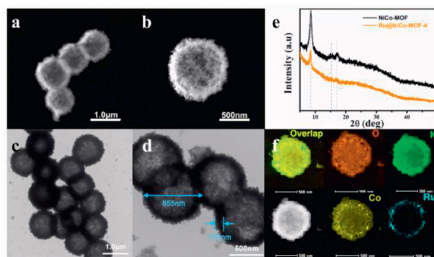
Fig. 9. HAADF-STEM images of (a) NiCo-MOF HPNs and (b) Ru@NiCo-MOF-4 HPNs. TEM images of (c) NiCo-MOF HPNs and (d) Ru@NiCo-MOF-4 HPNs. (e) XRD patterns. (f) Elemental mapping images of Ru@NiCo-MOF HPNs. Reproduced with permission [119]. Copyright 2021, ACS.
