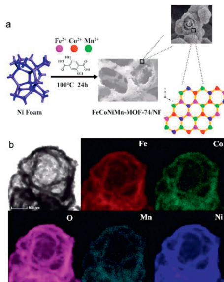
Fig. 4. Structure and characterization of materials. (a) In situ growth diagram of FeCoMnNi-MOF-74/NF. (b) TEM image and element map of FeCoMnNi-MOF-74/NF. Reproduced with permission [72]. Copyright 2021, ACS.
