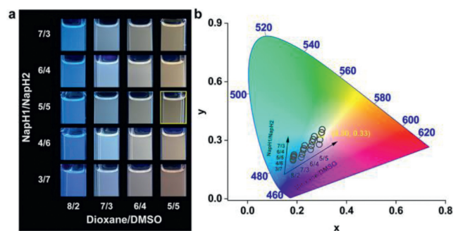
Fig. 3. (a) Luminescence photograph; and (b) CIE 1931 diagram of different mixing ratios of NapH1 and NapH2 and different ratios of dioxane and DMSO.
