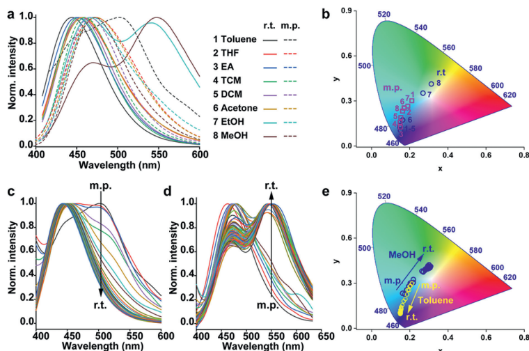
Fig. 4. (a) Fluorescence emission spectra; and (b) CIE 1931 diagrams of NapH1 at room temperature and melting point temperature. The fluorescence emission spectra from melting point temperature to room temperature of NapH1 in toluene (c); and methanol (d). (e) The corresponding CIE 1931 diagrams of (c) and (d).
