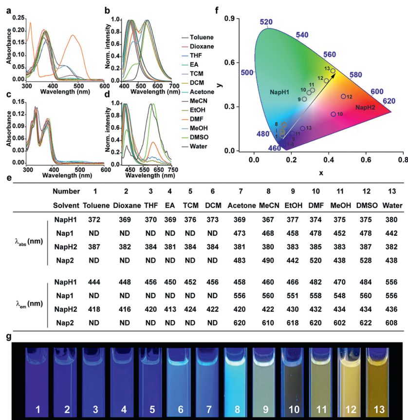
Fig. 1. The ultraviolet-visible (UV-vis) absorption spectra of NapH1 (a); and NapH2 (c) in different solvents. The fluorescence emission spectra of NapH1 (b); and NapH2 (d) in different solvents. (e) The spectral data table of NapH1 and NapH2 ; (f) the CIE 1931 diagram of NapH1 and NapH2 in different solvents; (g) the luminescence photographs of NapH1 in different solvents.
