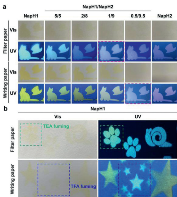
Fig. 5. The luminescence on the paper. (a) The color and luminescence of different mixing ratios of NapH1 and NapH2 on filter paper and writing paper respectively; (b) the color and luminescence of NapH1 on two kinds of paper and the change of color and luminescence after acid or base stimulation.
