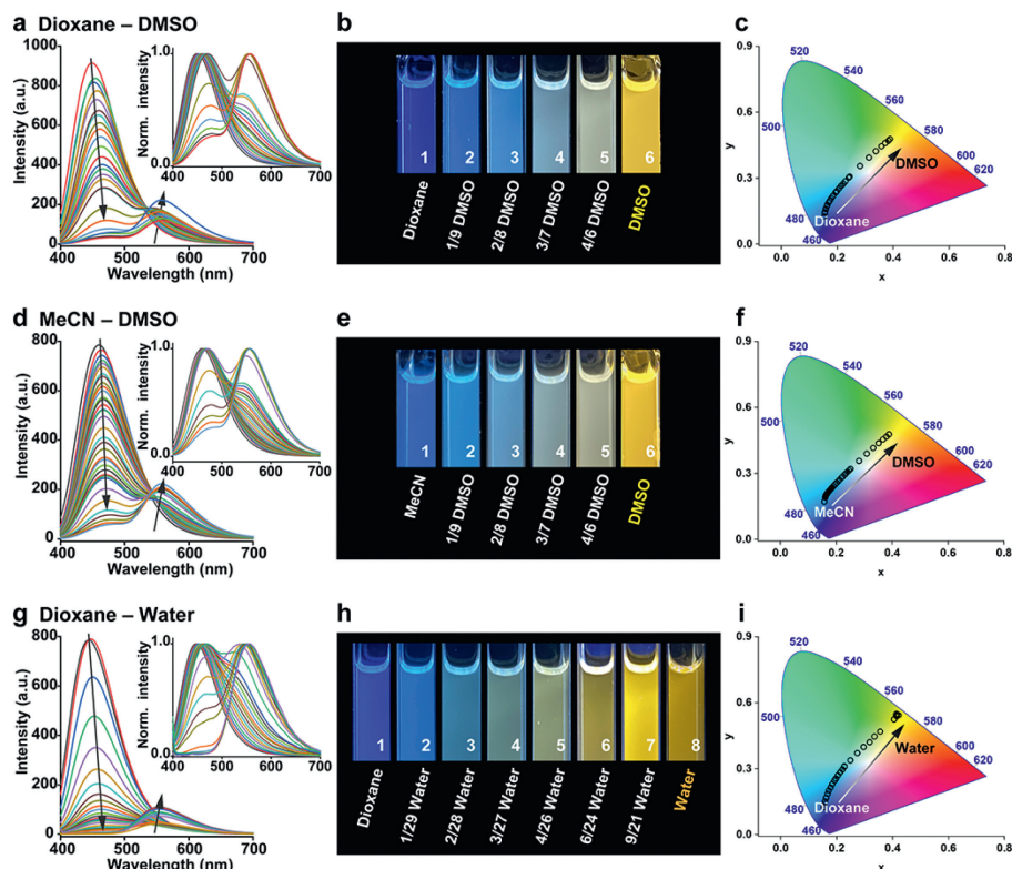
Fig. 2. The fluorescence emission spectra of NapH1 in (a) dioxane-DMSO; (d) MeCN-DMSO; and (g) dioxane-water system. The corresponding luminescence photographs of NapH1 in (b) dioxane-DMSO; (e) MeCN-DMSO; and (h) dioxane-water system. The CIE 1931 diagram of NapH1 in (c) dioxane-DMSO, (f) MeCN-DMSO, and (i) dioxane-water system.
