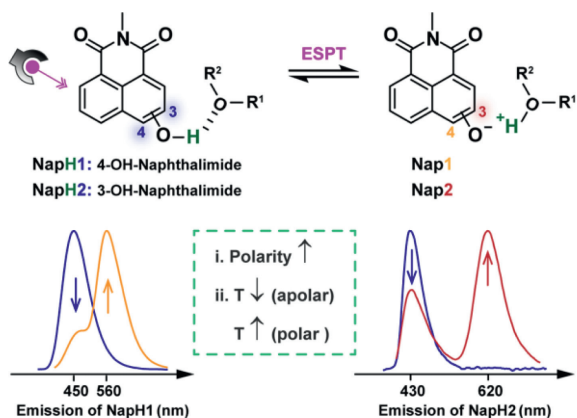
Scheme 1. Structure of NapH1 and NapH2 , and their ESPT properties and influencing factors. Nap1 and Nap2 is the deprotonation form of NapH1 and NapH2 .
