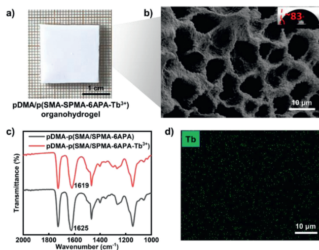
Fig. 1. Characterization of pDMA/p(SMA-SPMA-6APA-Tb 3+ ) organohydrogel. (a) Photograph and (b) cross-section SEM image and contact angle of pDMA/p(SMA-SPMA-6APA-Tb 3+ ) organohydrogel. (c) FT-IR spectra of pDMA/p(SMA-SPMA-6APA) organohydrogel that is absent or present of Tb 3+ ions. (d) EDS mapping of Tb 3+ in pDMA/p(SMA-SPMA-6APA-Tb 3+ ) organohydrogel.
