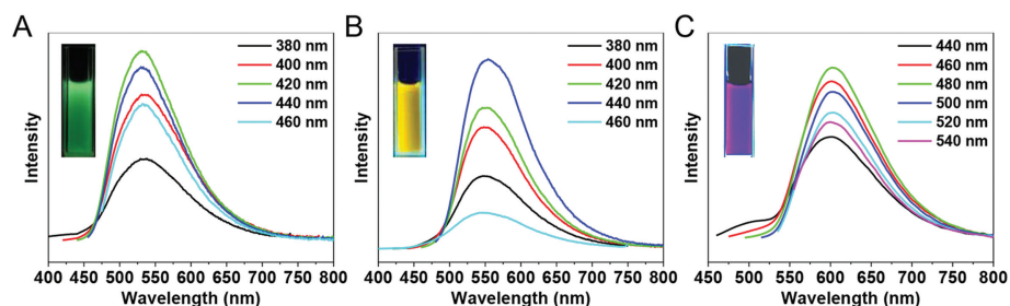
Fig. 4. PL emission spectra of the ethanol solutions of CDs under different wavelengths of excitation light from resorcinol (A), o -phenylenediamine (B) and p -phenylenediamine (C), with the inset photos under UV light.
