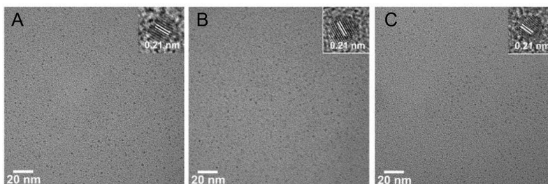
Fig. 3. TEM images of (A) G-CDs, (B) Y-CDs and (C) R-CDs, with their inset HRTEM images, respectively.
