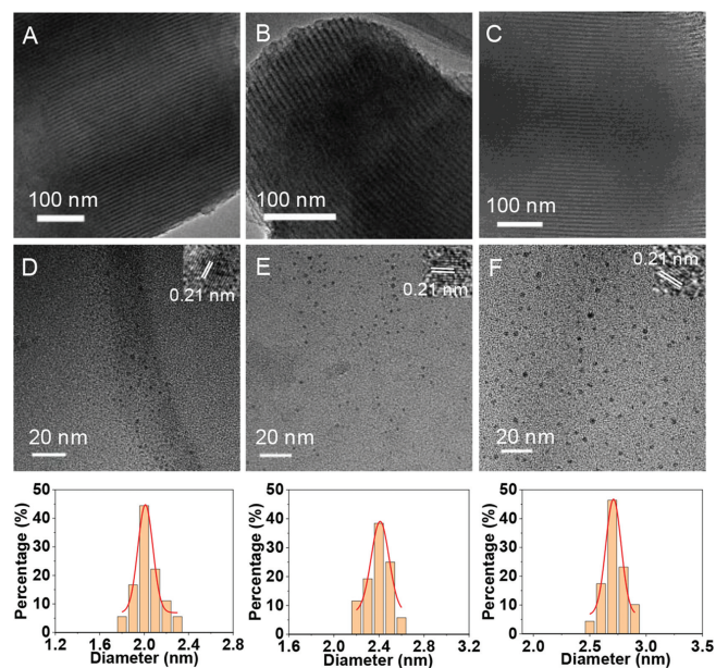
Fig. 1. TEM images of (A) SBA-15-A, (B) SBA-15-B and (C) SBA-15-C, respectively. TEM images and the corresponding particle size distributions of (D) Sample A, (E) Sample B and (F) Sample C, respectively.
