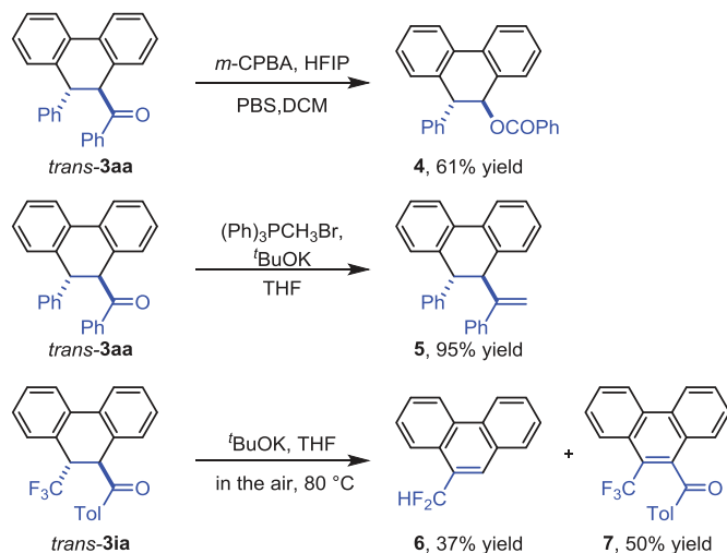
Scheme 4. Scale-up synthesis and derivatization.
