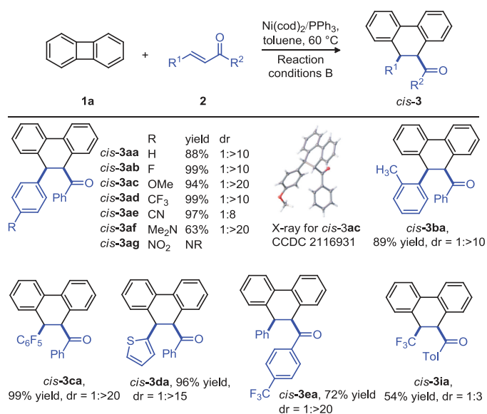
Scheme 3. Scope of substrates for the synthesis of cis -products. Reaction conditions B: 1a (0.1 mmol), 2 (0.1 mmol), Ni(cod) 2 (5 mol%), PPh 3 (10 mol%), in toluene (1.0 mL), 18 h, 60 °C, argon. dr = the ratio of trans / cis .
