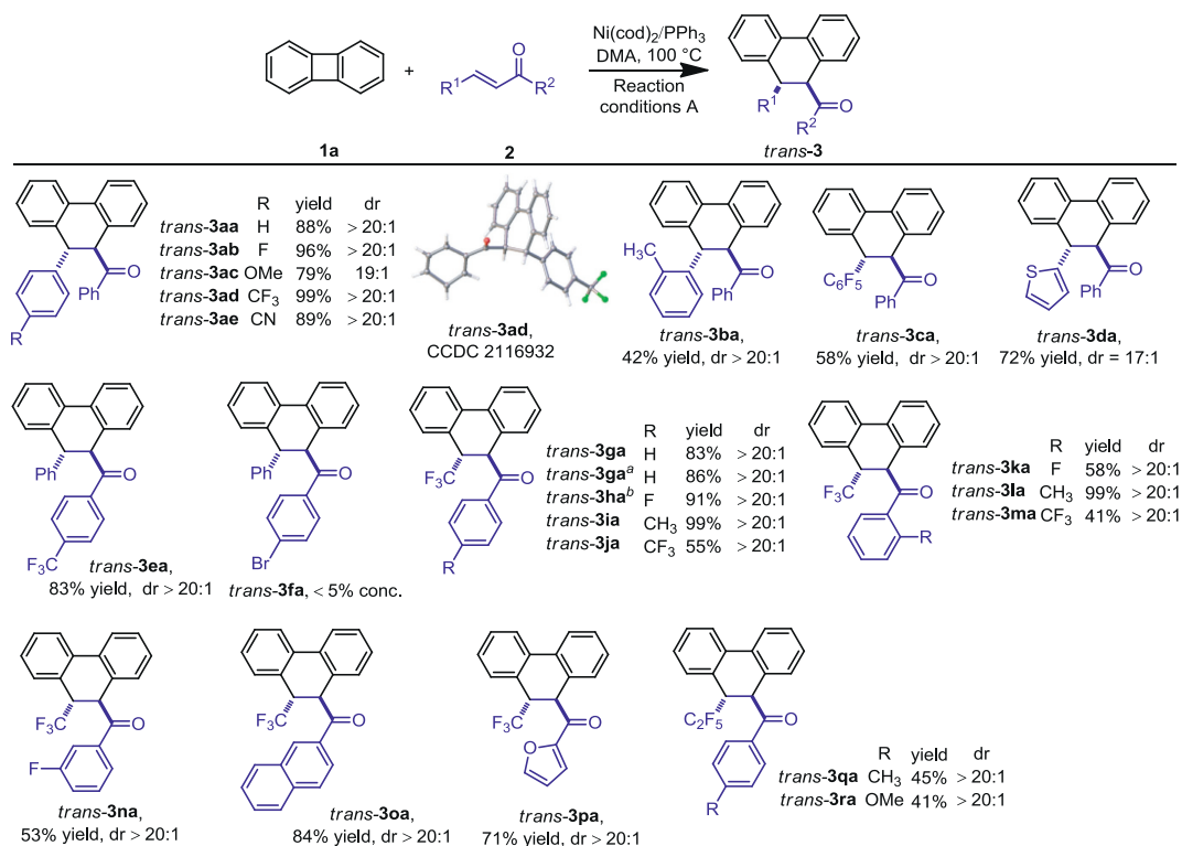
Scheme 2. Scope of substrates for the synthesis of trans -products. Reaction conditions A: Reaction conditions: 1a (0.1 mmol), 2 (0.1 mmol), Ni(cod) 2 (5 mol%), PPh 3 (10 mol%), in DMA (1.0 mL), 18 h, 100 °C, argon. a from the cis -enone substrates. b Ni(cod) 2 (5 mol%), PPh 3 (5 mol%) in DMA (1.0 mL), dr = the ratio of trans / cis .
