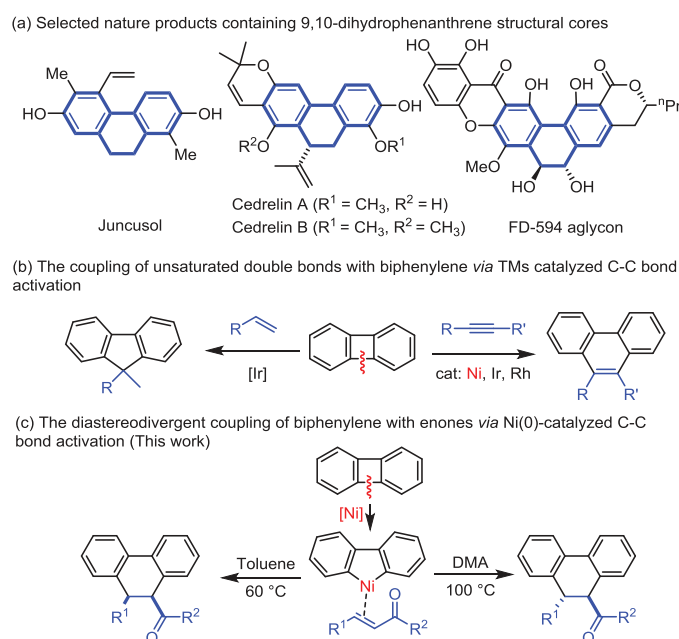
Scheme 1. Transition-metal catalyzed C–C functionalization of biphenylene.
