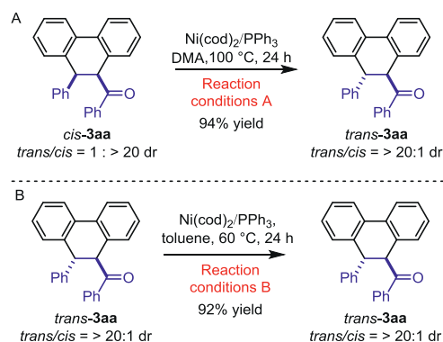
Scheme 6. Isomerization of the product.
