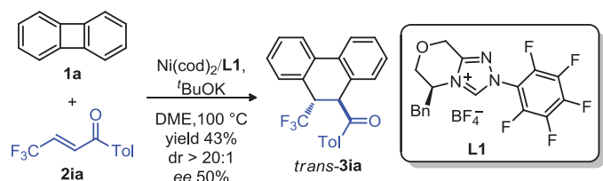
Scheme 5. Enantioselective coupling system.
