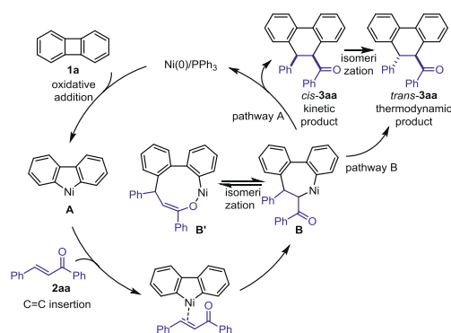
Scheme 7. Proposed mechanism.
