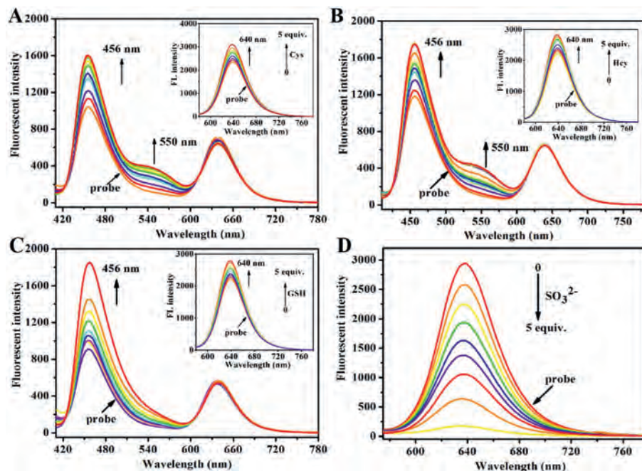
Fig. 1. Fluorescence spectra of PI-CO-NBD (10 \mu\text{mol/L} ) with (A) Cys (0–50 \mu\text{mol/L} ), (B) Hcy (0–50 \mu\text{mol/L} ), (C) GSH (0–50 \mu\text{mol/L} ), (D) \text{SO}_3^{2-} (0–50 \mu\text{mol/L} ) in the PBS buffer (pH 7.4, containing 20% \text{CH}_3\text{CN} , v/v). \lambda_{\text{ex}} = 395 \text{ nm} , Ex/Em slit: 5/2 nm.
