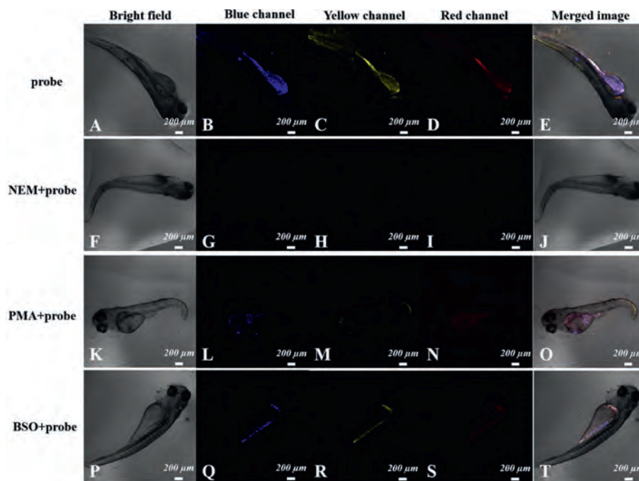
Fig. 4. Fluorescence imaging of Cys/Hcy and GSH with three-channel in zebrafish: (A–E): Zebrafish were treated with the PI-CO–NBD probe; (F–T): Cells were respectively pretreated with NEM (1 mmol/L), PMA (1 \mu g/mL), or BSO (100 \mu mol/L) for 30 min and then incubated with PI-CO–NBD (10 \mu mol/L) for 10 min. Blue channel: \lambda_{\text{ex}} = 405 nm, \lambda_{\text{em}} = 450\text{--}510 nm; yellow channel: \lambda_{\text{ex}} = 451 nm, \lambda_{\text{em}} = 520\text{--}580 nm; red channel: \lambda_{\text{ex}} = 561 nm, \lambda_{\text{em}} = 610\text{--}670 nm.
