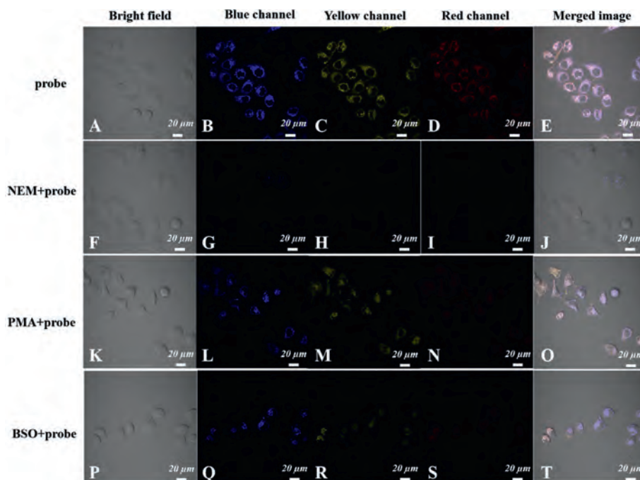
Fig. 3. Fluorescence images of endogenous thiols in living HeLa cell. (A–E): Cells were treated with the PI-CO-NBD probe, (F–T): Cells were respectively pretreated with NEM (1 mmol/L), PMA (1 \mu\text{g/mL} ), or BSO (100 \mu\text{mol/L} ) for 30 min and then incubated with PI-CO-NBD (10 \mu\text{mol/L} ) for 10 min. Blue channel: \lambda_{\text{ex}} = 405 \text{ nm} , \lambda_{\text{em}} = 450\text{--}510 \text{ nm} ; yellow channel: \lambda_{\text{ex}} = 451 \text{ nm} , \lambda_{\text{em}} = 520\text{--}580 \text{ nm} ; red channel: \lambda_{\text{ex}} = 561 \text{ nm} , \lambda_{\text{em}} = 610\text{--}670 \text{ nm} .
