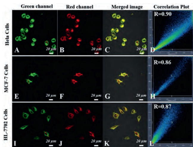
Fig. 2. Intracellular localization of PI-CO-NBD in living MCF-7, HL-7702 and HeLa cells. (A, E, I) All the tested cells were prestained with MitoTracker Green FM (1 \mu\text{mol/L} ), ( \lambda_{\text{ex}} = 488 \text{ nm} and \lambda_{\text{em}} range: 498–651 nm). (B, F, J) All the tested cells were treated with PI-CO-NBD (10 \mu\text{mol/L} ). \lambda_{\text{ex}} = 565 \text{ nm} and \lambda_{\text{em}} range 610–670 nm. (C, G, K) Merged images. (D, H, L) Intensity profiles of regions of interest.
