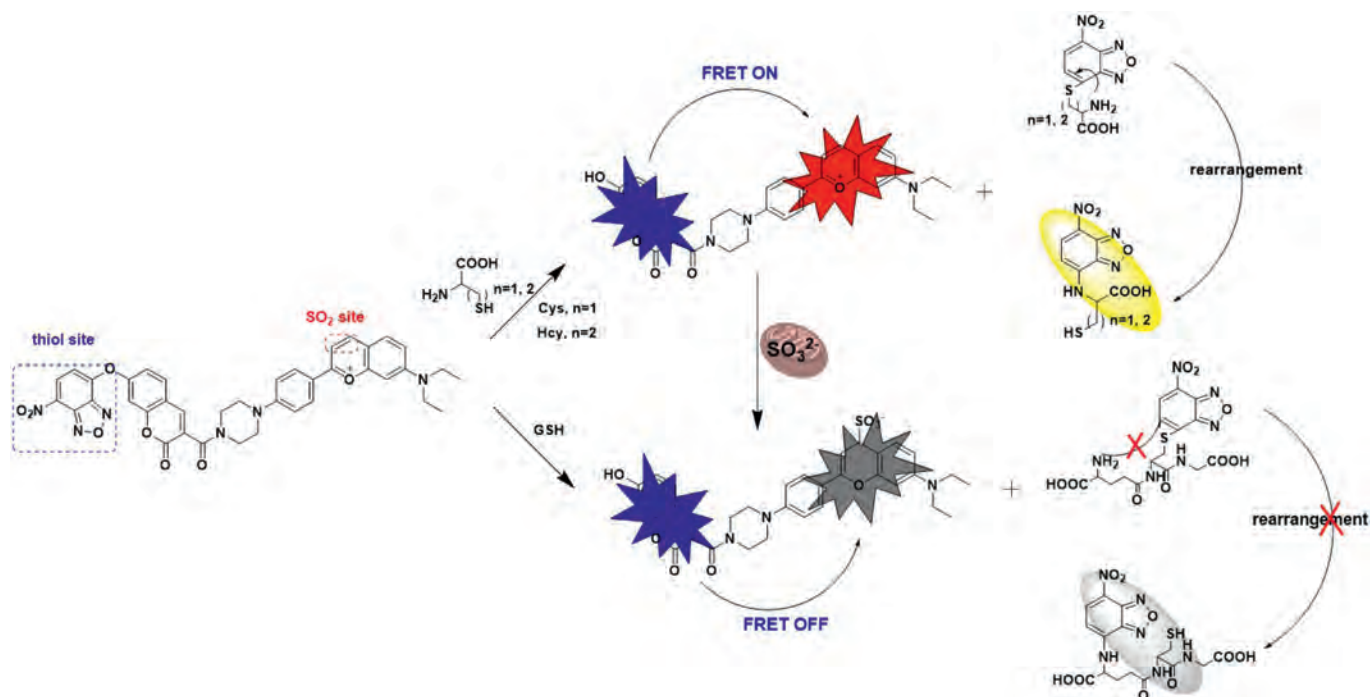
Scheme 2. Response mechanisms of PI-CO-NBD with Cys/Hcy/GSH and \text{SO}_2 .
