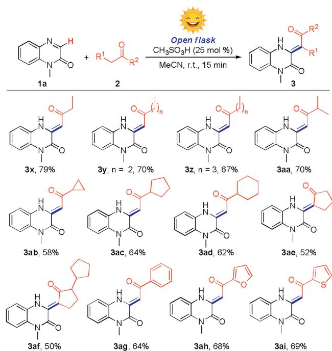
Scheme 3. Substrate scope of methyl ketones. Reaction conditions: 1a (0.2 mmol), 2 (2.0 equiv.), CH 3 SO 3 H (25 mol%), MeCN (1.0 mL), open flask, sunlight, room temperature, 15 min. Isolated yields.
