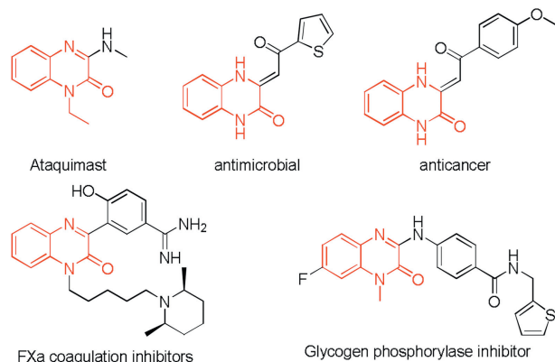
Fig. 1. Examples of quinoxalin-2(1H)-one skeleton-based bioactive molecules.
