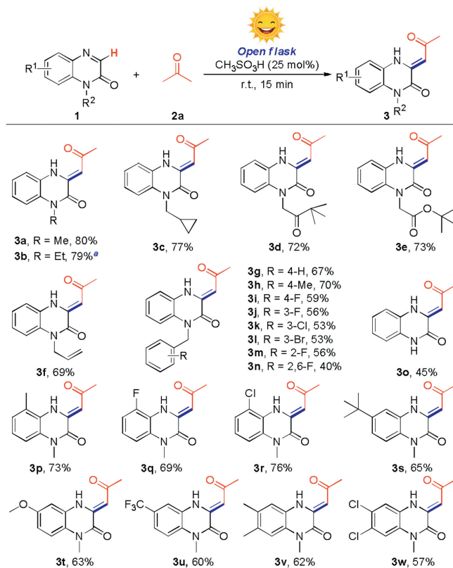
Scheme 2. Substrate scope of quinoxalin-2(1H)-ones. Reaction conditions: 1 (0.2 mmol), 2a (1.0 mL), \text{CH}_3\text{SO}_3\text{H} (25 mol%), open flask, sunlight, room temperature, 15 min. Isolated yields. a Reaction was performed on a 1 mmol scale.
