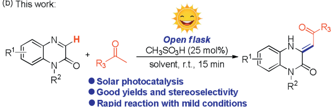
Scheme 1. Modification of quinoxalin-2(1H)-ones by C-H functionalization.
