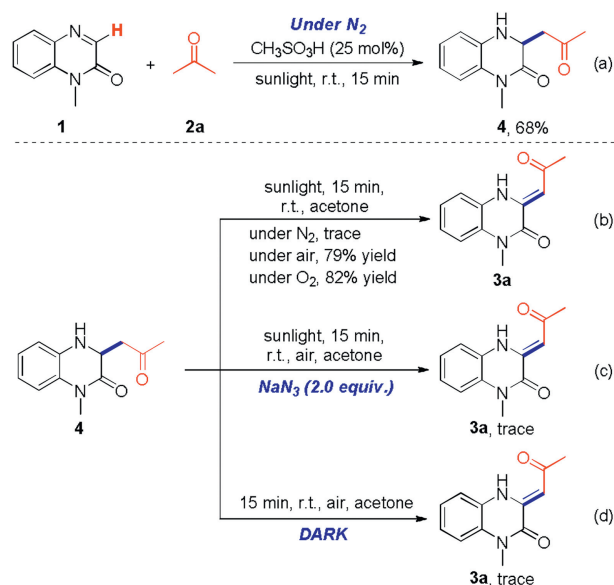
Scheme 5. Control experiments.
