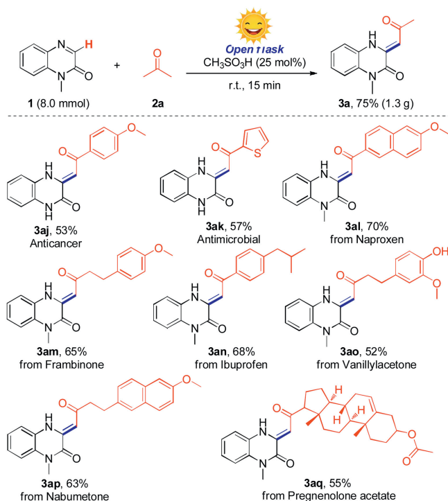
Scheme 4. Gram-scale synthesis and application. Reaction conditions: 1a (0.2 mmol), 2 (2.0 equiv.), CH 3 SO 3 H (25 mol%), MeCN (1.0 mL), open flask, sunlight, room temperature, 15 min. Isolated yields.
