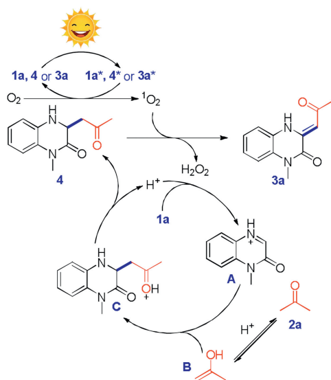
Scheme 6. Plausible mechanism.
