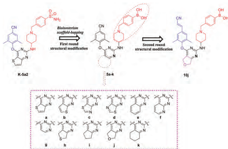
Fig. 3. Design and optimization of the boronic acid-containing DAPY derivatives.
