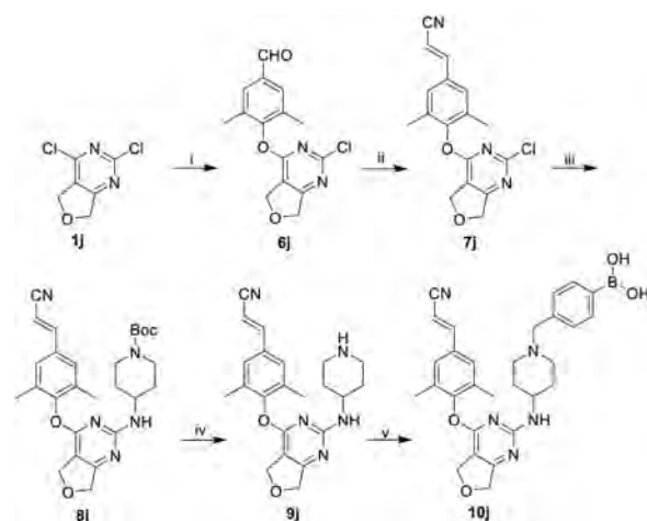
Scheme 2. Synthesis of 10j . Reagents and conditions: i) 4-hydroxy-3,5-dimethylbenzaldehyde, K_2CO_3 , DMF, r.t.; ii) (EtO)_2P(O)CH_2CN , t-BuOK , THF, 0^\circ C to r.t.; iii) BINAP, Pd_2(dba)_3 , Cs_2CO_3 , 1,4-dioxane, 90^\circ C , N_2 ; iv) TFA, DCM, r.t.; v) (4-(chloromethyl)phenyl)boronic acid, K_2CO_3 , DMF, r.t.
