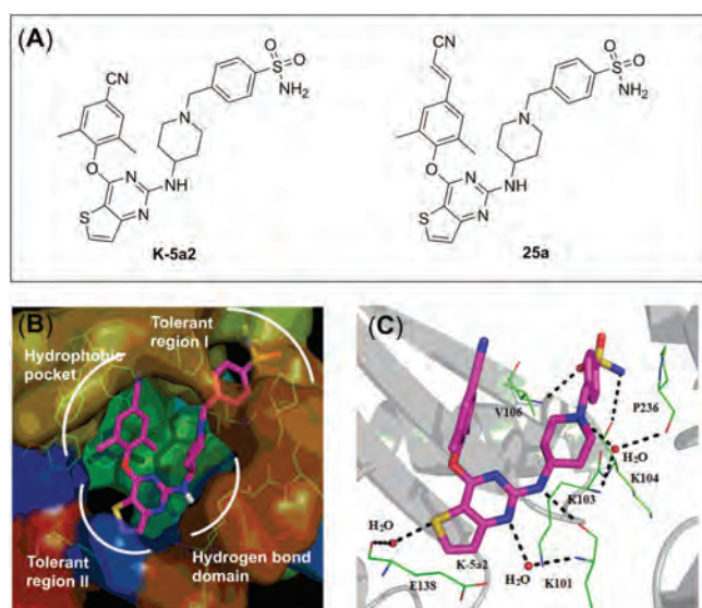
Fig. 2. (A) Chemical structures of our previously reported potent HIV-1 NNRTIs; (B) The co-crystal structure of K-5a2 /RT complexes (PDB code: 6c0j) and the four-point pharmacophore model; (C) The detailed interactions with WT RT of K-5a2 .
