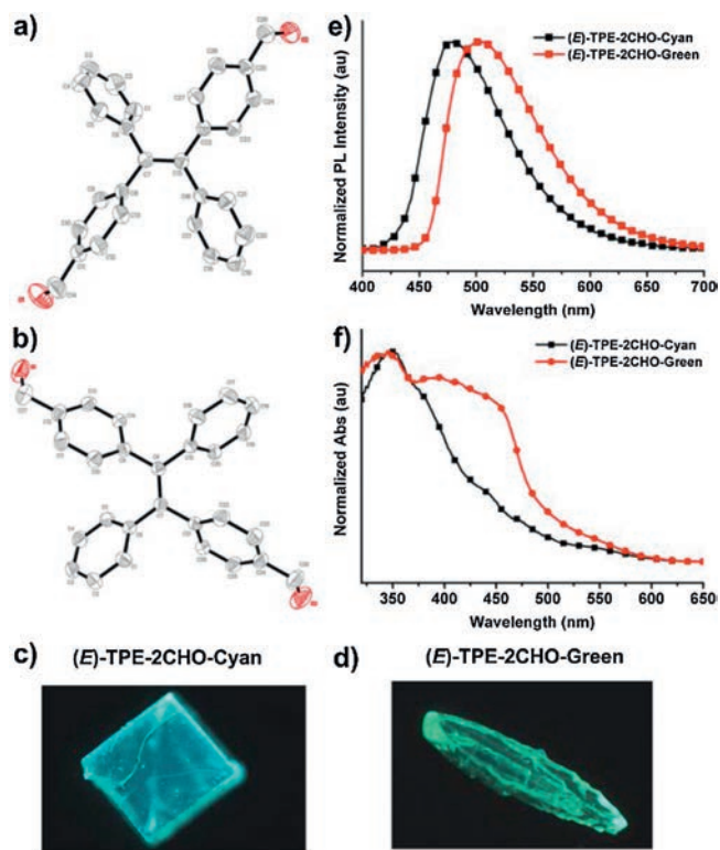
Fig. 2. (a, b) ORTEP drawings (50% probability ellipsoids) and the numbering schemes for the two polymorphs. (c, d) PL images of the two crystals taken under a 365 nm UV light. (e, f) PL spectra and UV-vis reflection spectra of the two polymorphs.
