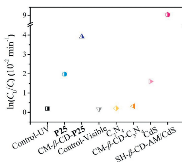
Fig. 2. The apparent rate constant ( K_a ) of different cyclodextrin modified photooxidation systems for photocatalytic degradation of bisphenol A. Reaction condition: [BPA]_0 = 20 mg/L. [photocatalyst] = 1 mg/mL, pH_{ini} = 6.8 , T = 298 \pm 1 K.
