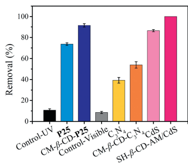
Fig. 1. The removal of bisphenol A by different photocatalytic oxidation systems. Reaction condition: [BPA]_0 = 20 mg/L. [photocatalyst] = 1 mg/mL, pH_{ini} = 6.8 , T = 298 \pm 1 K.
