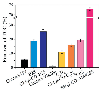
Fig. 3. TOC removal of different cyclodextrin modified photooxidation systems for photocatalytic degradation of bisphenol A. Reaction condition: [BPA]_0 = 20 \text{ mg/L} , [\text{photocatalyst}] = 1 \text{ mg/mL} , \text{pH}_{\text{ini}} = 6.8 , T = 298 \pm 1 \text{ K} .
