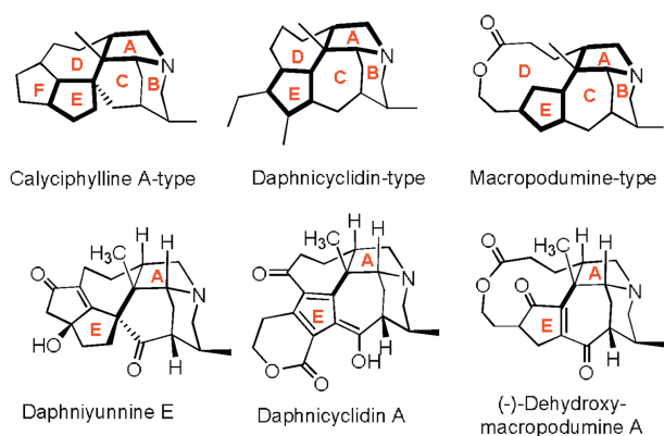
Fig. 1. Representative structures of calyciphylline A-type, daphnicyclidin-type and macropodumine-type alkaloids.
