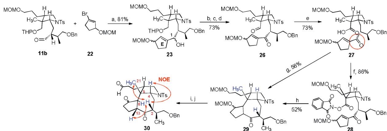
Scheme 5. Construction of ACE tricyclic of dehydroxymacro-podumine A by decarboxylation conjugate addition. Reagents and conditions: (a) 22 , t -BuLi, THF, -78^{\circ}\text{C} ; (b) DMP, DCM, 25^{\circ}\text{C} ; (c) 1 mol/L HCl, MeOH, 25^{\circ}\text{C} , 24 h; (d) DMP, DCM, 25^{\circ}\text{C} ; (e) \text{NaH}_2\text{PO}_4 , \text{NaClO}_2 , t -BuOH/ \text{CH}_3\text{CN}/\text{H}_2\text{O} = 2:2:1 , 0^{\circ}\text{C} – 25^{\circ}\text{C} ; (f) N -hydroxy-phthalimide, DIC, THF, 25^{\circ}\text{C} , 24 h; (g) 1 mol% \text{Ir}[\text{dF}(\text{CF}_3)\text{ppy}]_2(\text{dtbbpy})\text{PF}_6 , \text{K}_2\text{HPO}_4 , DMF, 25^{\circ}\text{C} , 26 W GL, 16 h; (h) diethyl 1,4-dihydro-2,6-dimethyl-3,5-pyridine-dicarboxylate, \text{CH}_2\text{Cl}_2 , DIPEA, blue light, [\text{Ru}(\text{bpy})_3](\text{BF}_4)_2 , 25^{\circ}\text{C} , 2 h; (i) 3 mol/L HCl, MeOH, 12 h; (j) DMP, DCM, 25^{\circ}\text{C} .
